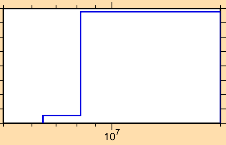
\sigma vs. E for ^{134}\text{Pm}(\text{mt117})
