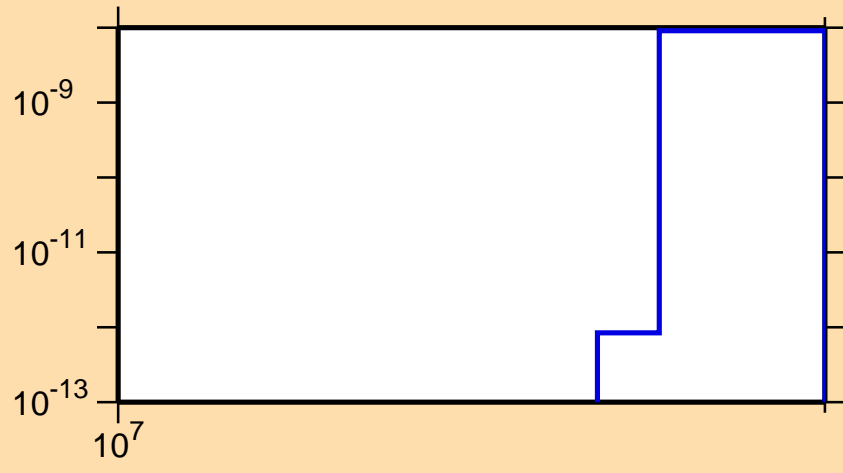
\sigma vs. E for ^{135}\text{Pm}(n,nt)
