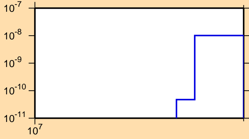
\sigma vs. E for ^{135}\text{Pm}(n,pt)
