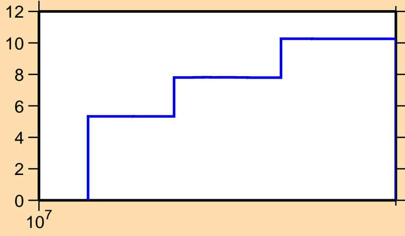
\Delta\sigma/\sigma vs. E for ^{135}\text{Pm}(n,\text{tot.})
