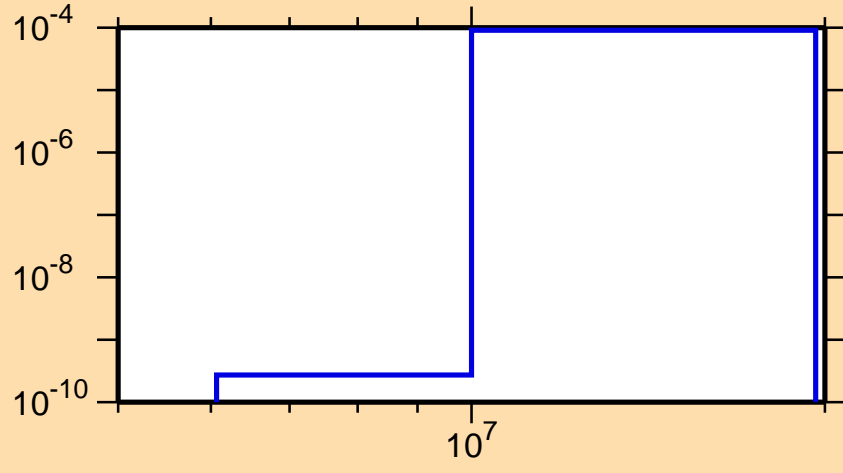
\sigma vs. E for ^{135}\text{Pm} (mt 45)
