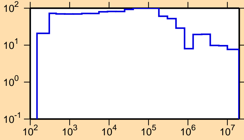
\Delta\sigma/\sigma vs. E for ^{135}\text{Pm}(n,e.l.)
