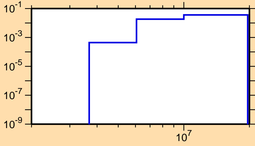
\sigma vs. E for ^{135}\text{Pm}(n,n\alpha)
