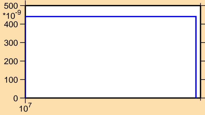
\sigma vs. E for ^{135}\text{Pm}(n,\text{nd})
