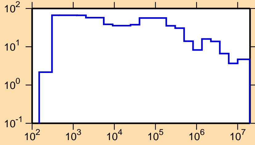
\Delta\sigma/\sigma vs. E for ^{135}\text{Pm}(n,\text{tot.})
