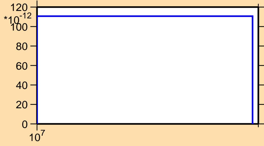
\sigma vs. E for ^{135}\text{Pm}(n,pt)
