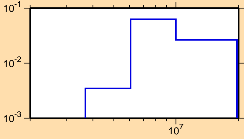
\sigma vs. E for ^{135}\text{Pm}(n,n\text{cont.})
