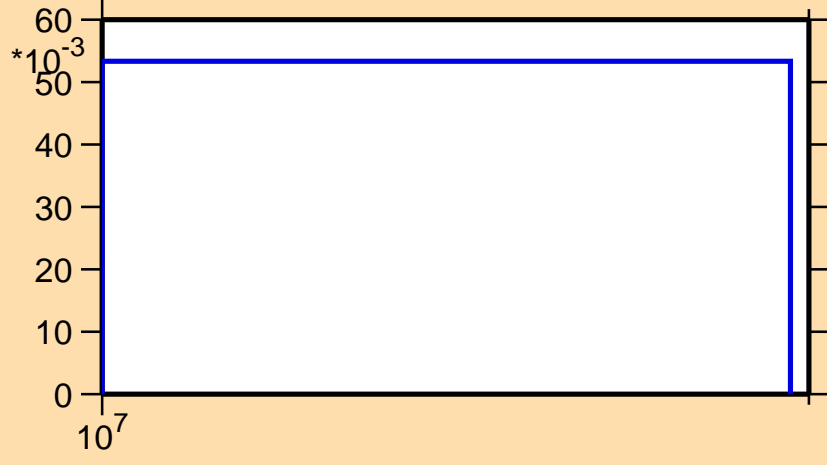
\sigma vs. E for ^{135}\text{Pm}(n,2n)
