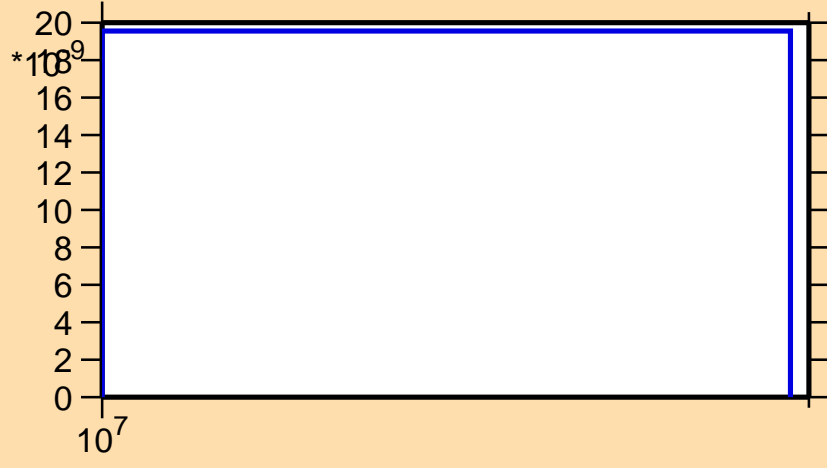
\sigma vs. E for ^{135}\text{Pm}(n,2n\alpha)
