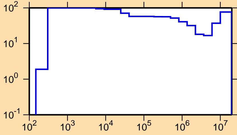
\Delta\sigma/\sigma vs. E for ^{135}\text{Pm}(n,p)
