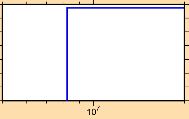
\sigma vs. E for ^{135}\text{Pm}(n,nt)
