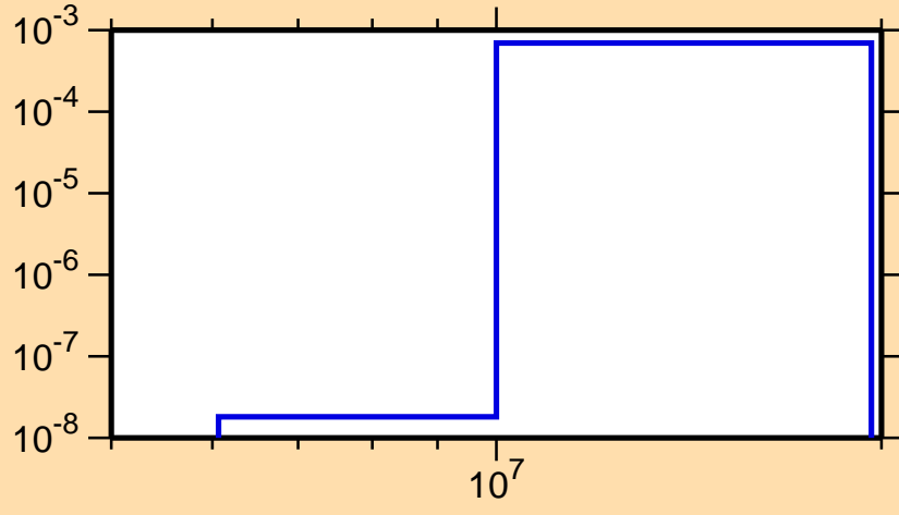
\sigma vs. E for ^{136}\text{Pm}(n,t)
