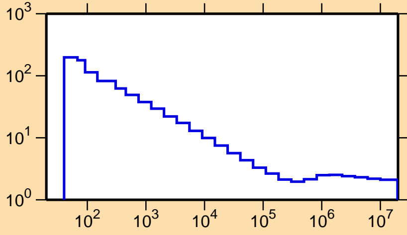
\sigma vs. E for ^{136}\text{Pm}(n,\text{nonel.})
