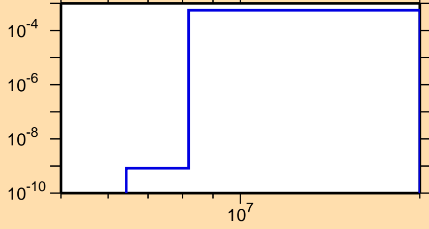
\sigma vs. E for ^{136}\text{Pm}(n,t)
