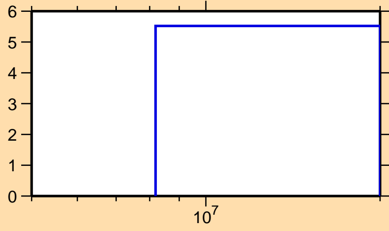
\Delta\sigma/\sigma vs. E for ^{136}\text{Pm}(n,\text{el.})
