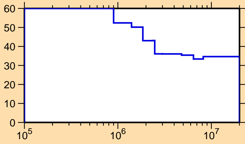
\Delta\sigma/\sigma vs. E for ^{136}\text{Pm}(n,n_1)
