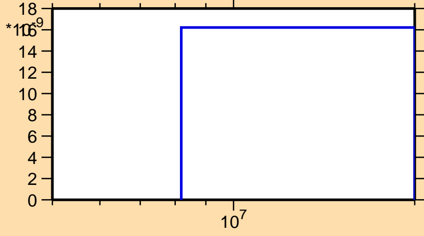
\sigma vs. E for ^{136}\text{Pm}(n,pt)
