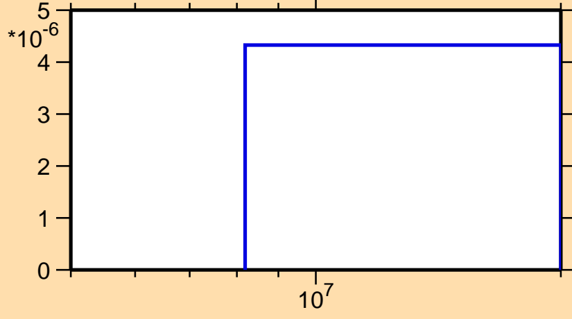
\sigma vs. E for ^{136}\text{Pm}(n,nd)
