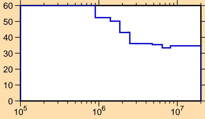
\Delta\sigma/\sigma vs. E for ^{136}\text{Pm}(n,n_1)
