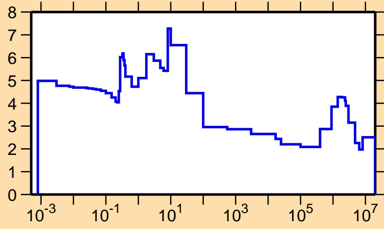
\sigma vs. E for ^{136}\text{Pm}(n,\text{el.})
