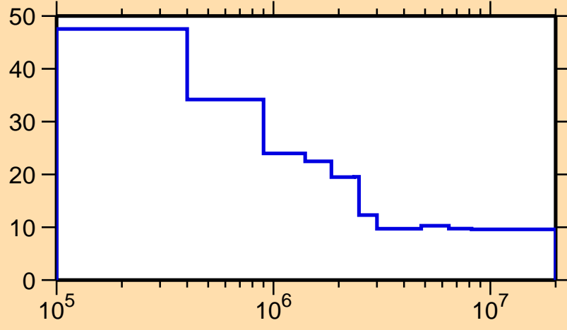
\Delta\sigma/\sigma vs. E for ^{136}\text{Pm}(n,\text{nonel.})
