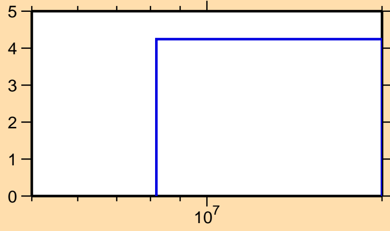
\Delta\sigma/\sigma vs. E for ^{136}\text{Pm}(n,\text{tot.})
