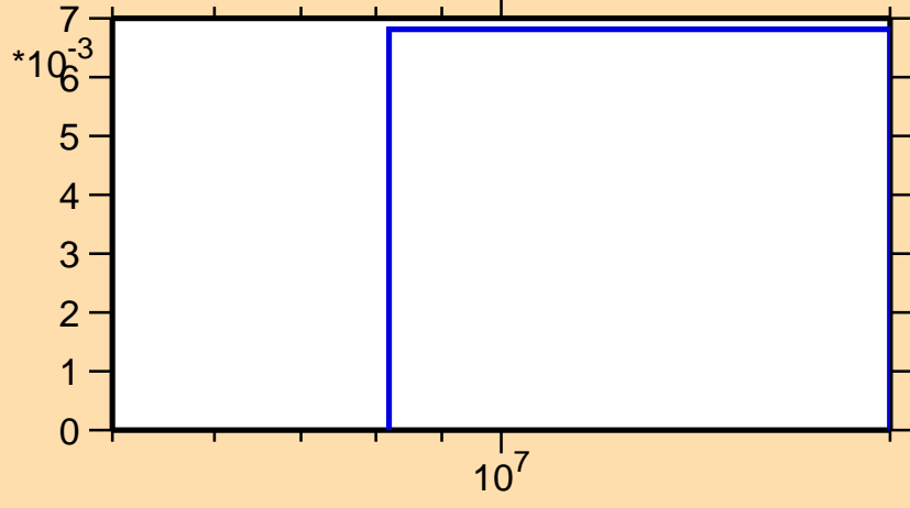
\sigma vs. E for ^{136}\text{Pm}(n,2np)
