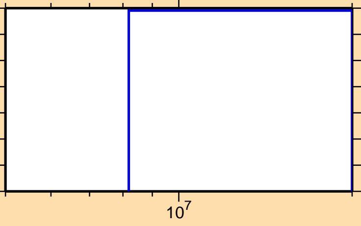
\sigma vs. E for ^{136}\text{Pm}(n,2n)
