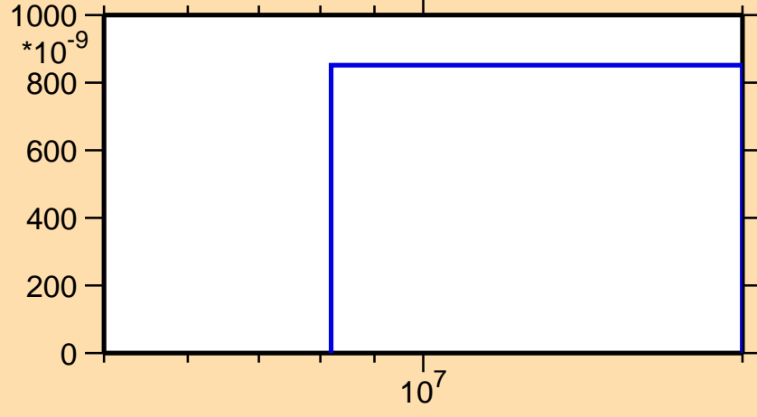
\sigma vs. E for ^{136}\text{Pm}(n,pd)
