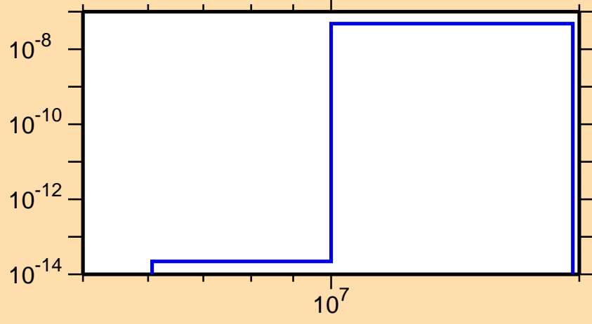
\sigma vs. E for ^{137}\text{Pm} (mt117)
