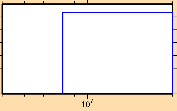
\sigma vs. E for ^{137}\text{Pm}(n,2n\alpha)
