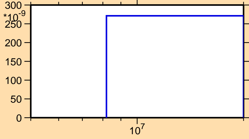
\sigma vs. E for ^{137}\text{Pm}(n,nd)
