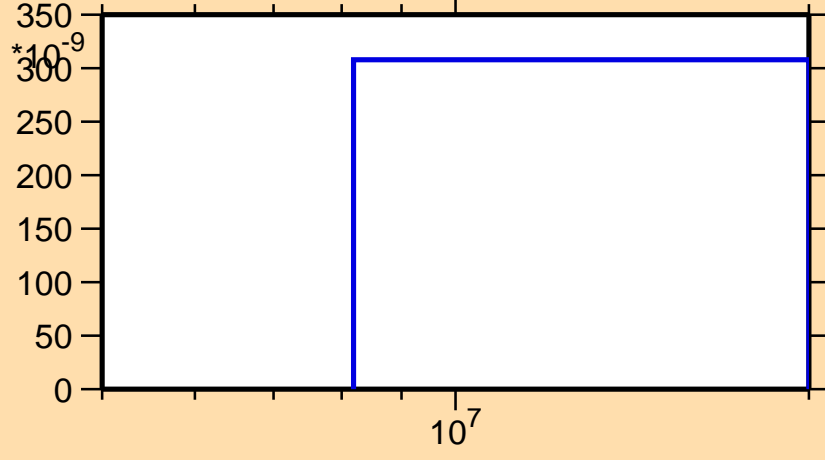
\sigma vs. E for ^{137}\text{Pm}(n,pd)
