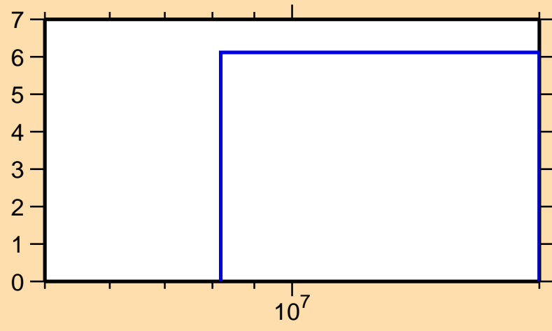
\Delta\sigma/\sigma vs. E for ^{137}\text{Pm}(n,el.)
