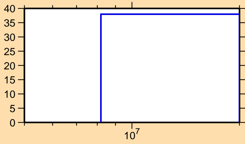
\Delta\sigma/\sigma vs. E for ^{138}\text{Pm}(n,2n)
