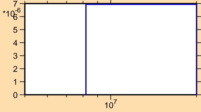
\sigma vs. E for ^{138}\text{Pm}(n,nd)
