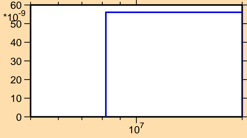
\sigma vs. E for ^{138}\text{Pm}(n,pd)
