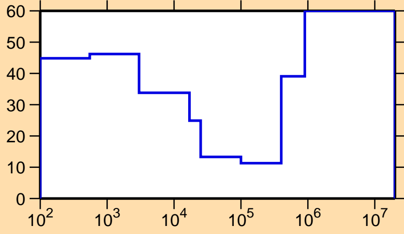
\Delta\sigma/\sigma vs. E for ^{138}\text{Pm}(n,p)
