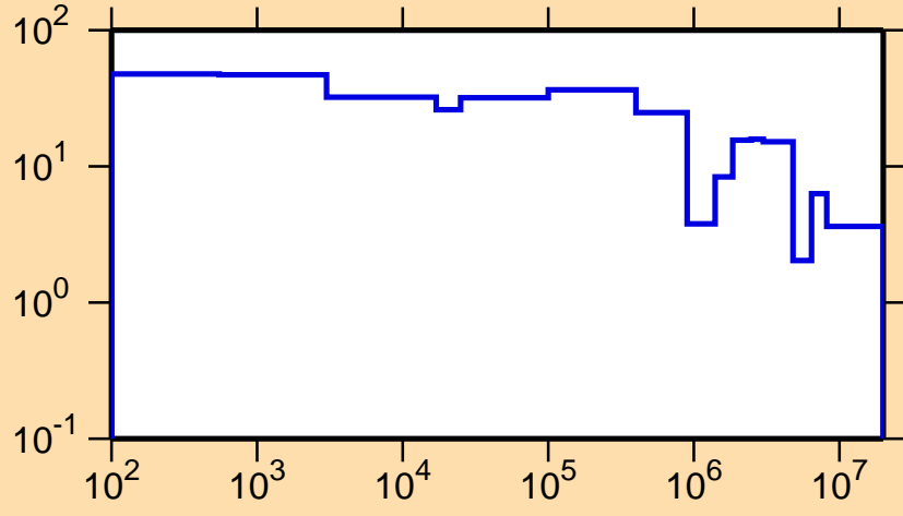
\Delta\sigma/\sigma vs. E for ^{138}\text{Pm}(n,el.)
