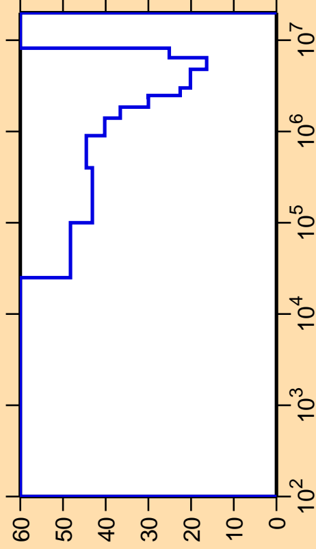
\Delta\sigma/\sigma vs. E for ^{138}\text{Pm}(n,\text{inel.})
