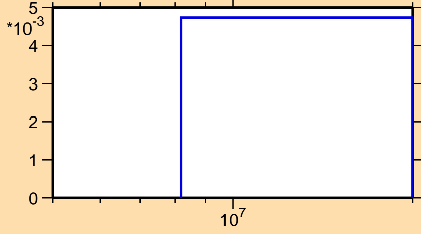
\sigma vs. E for ^{138}\text{Pm}(n,2np)
