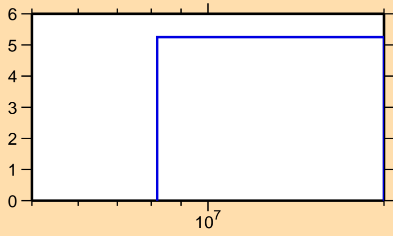
\Delta\sigma/\sigma vs. E for ^{138}\text{Pm}(n,\text{nonel.})
