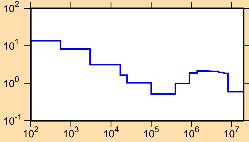
\sigma vs. E for ^{138}\text{Pm}(n,\text{inel.})
