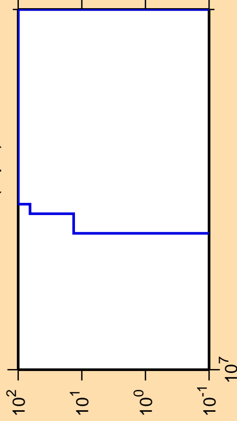
\Delta\sigma/\sigma vs. E for ^{139}\text{Pm}(n,pd)
