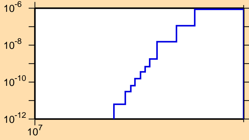
\sigma vs. E for ^{139}\text{Pm}(n,pd)
