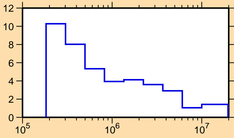
\Delta\sigma/\sigma vs. E for ^{139}\text{Pm}(n,\text{tot.})
