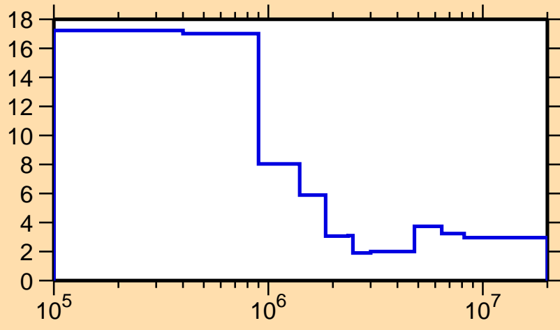
\Delta\sigma/\sigma vs. E for ^{139}\text{Pm}(n,\text{nonel.})
