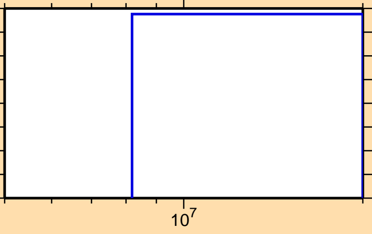
\sigma vs. E for ^{139}\text{Pm}(n,2n\alpha)
