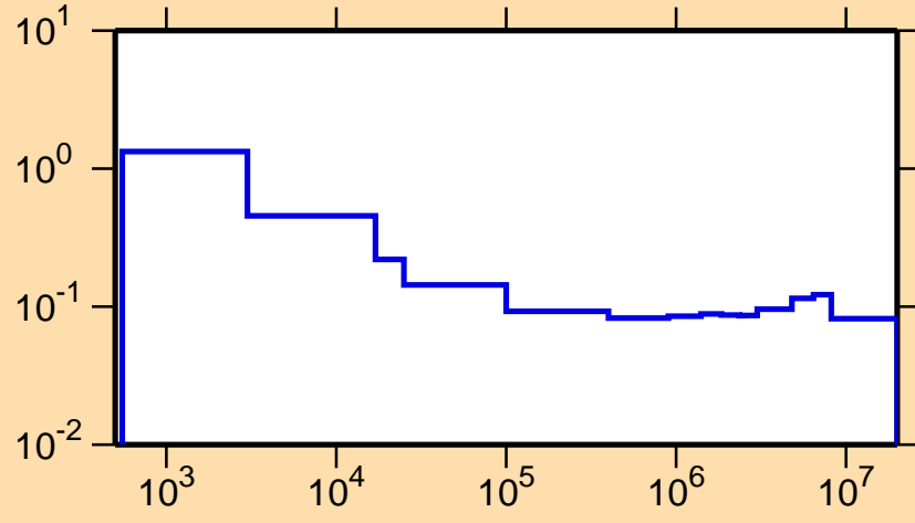
\sigma vs. E for ^{139}\text{Pm}(n,p)
