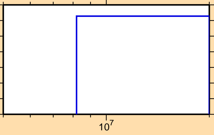
\sigma vs. E for ^{139}\text{Pm}(n,3n)
