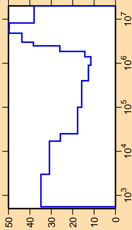
\Delta\sigma/\sigma vs. E for ^{139}\text{Pm}(n,\gamma)
