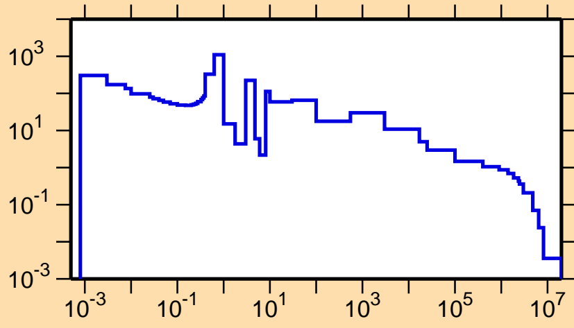
\sigma vs. E for ^{139}\text{Pm}(n,\gamma)
