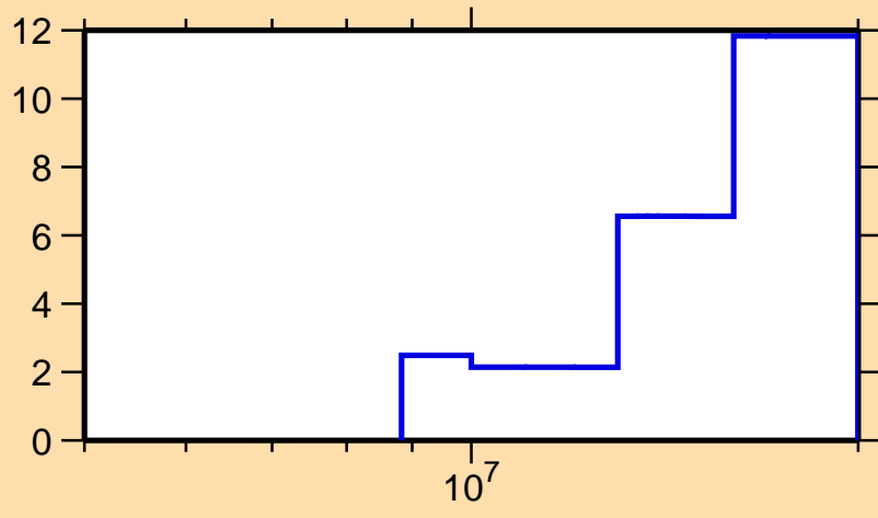
\Delta\sigma/\sigma vs. E for ^{140}\text{Pm}(n,\text{tot.})
