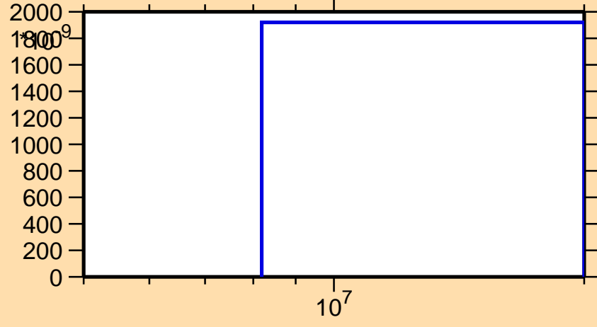
\sigma vs. E for ^{140}\text{Pm}(n,nd)
