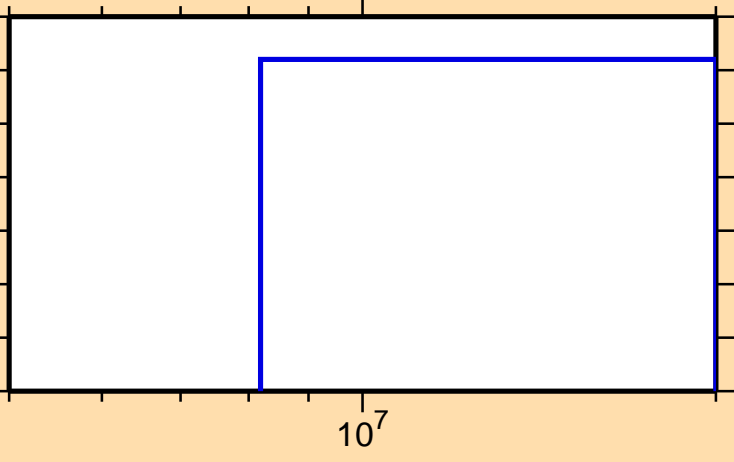
\sigma vs. E for ^{140}\text{Pm} (mt 45)
