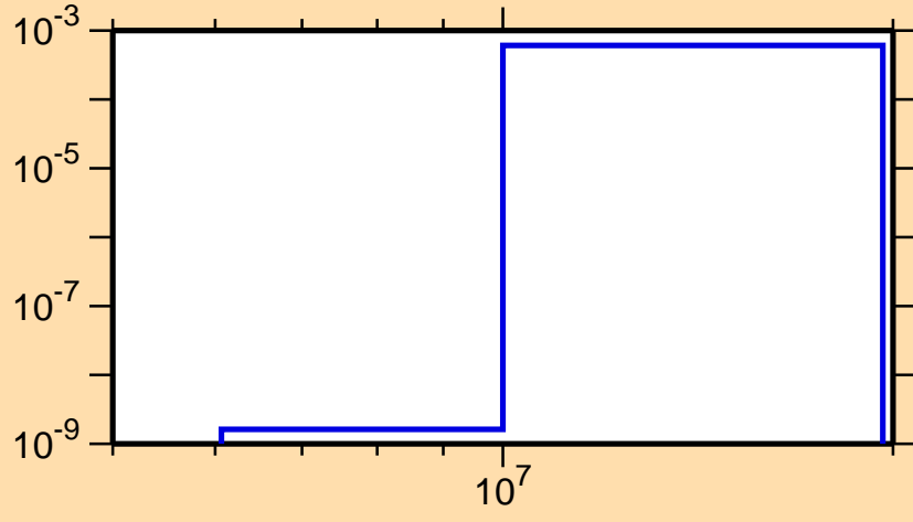
\sigma vs. E for ^{140}\text{Pm}(n,t)
