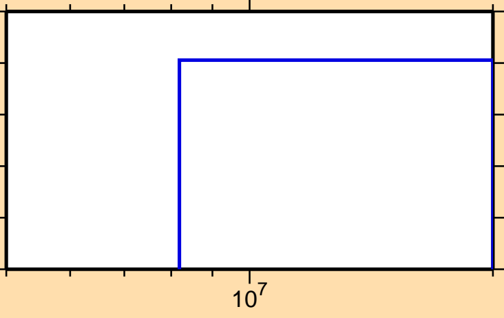
\sigma vs. E for ^{140}\text{Pm}(n,nd)
