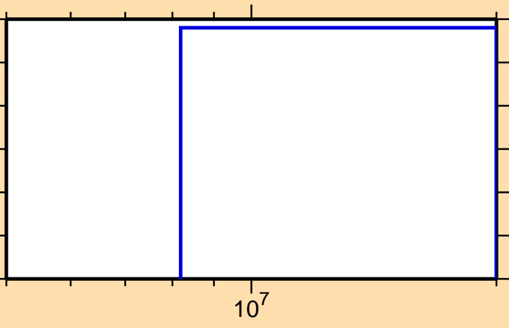
\sigma vs. E for ^{140}\text{Pm} (mt 45)
