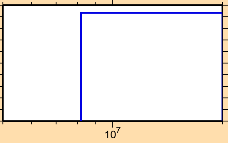
\sigma vs. E for ^{140}\text{Pm}(n,\text{He}3)
