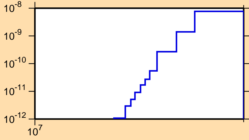
\sigma vs. E for ^{141}\text{Pm}(\text{mt117})
