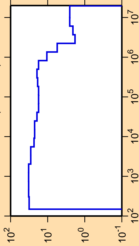
\Delta\sigma/\sigma vs. E for ^{141}\text{Pm}(n,\text{nonel.})
