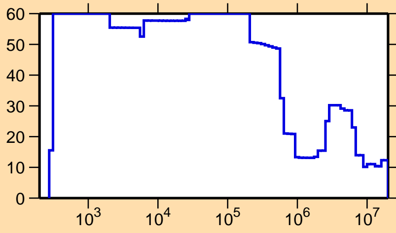
\Delta\sigma/\sigma vs. E for ^{142}\text{Pm}(n,el.)
