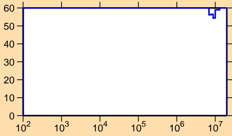
\Delta\sigma/\sigma vs. E for ^{143}\text{Pm}(n,\gamma)
