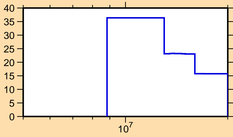
\Delta\sigma/\sigma vs. E for ^{143}\text{Pm}(n,2n)
