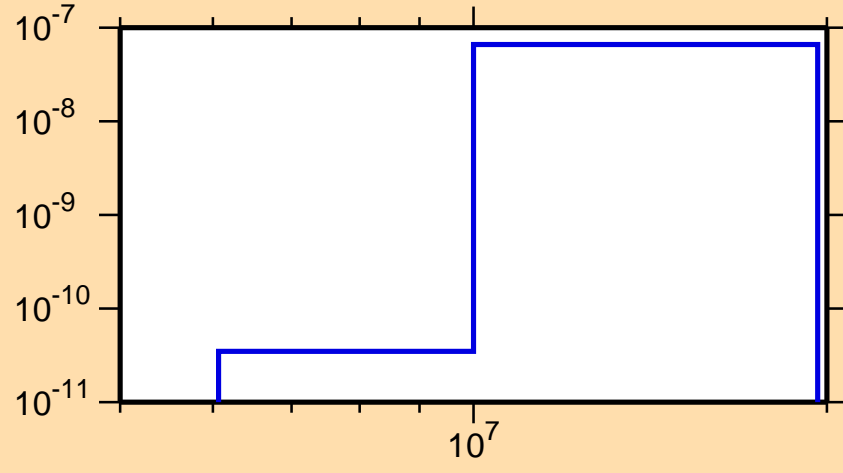
\sigma vs. E for ^{143}\text{Pm}(n,p\alpha)
