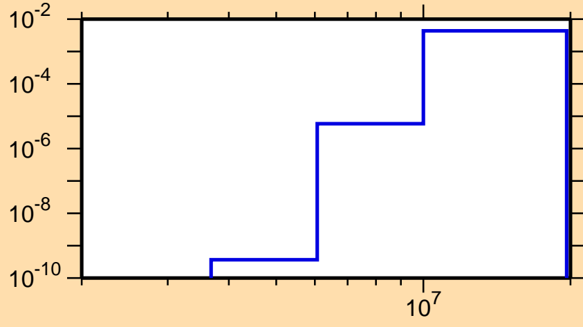
\sigma vs. E for ^{143}\text{Pm}(n,d)
