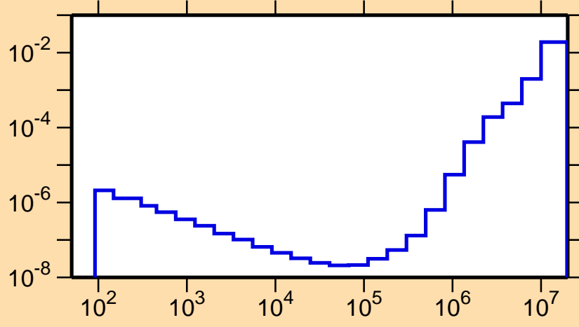
\sigma vs. E for ^{143}\text{Pm}(n,p)
