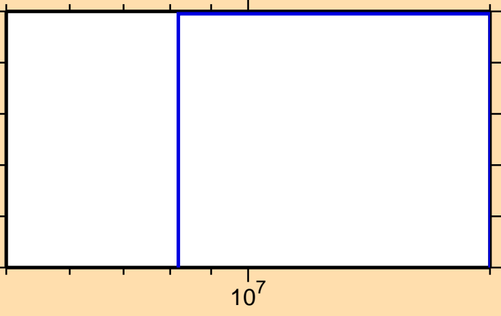
\sigma vs. E for ^{143}\text{Pm}(n,2np)
