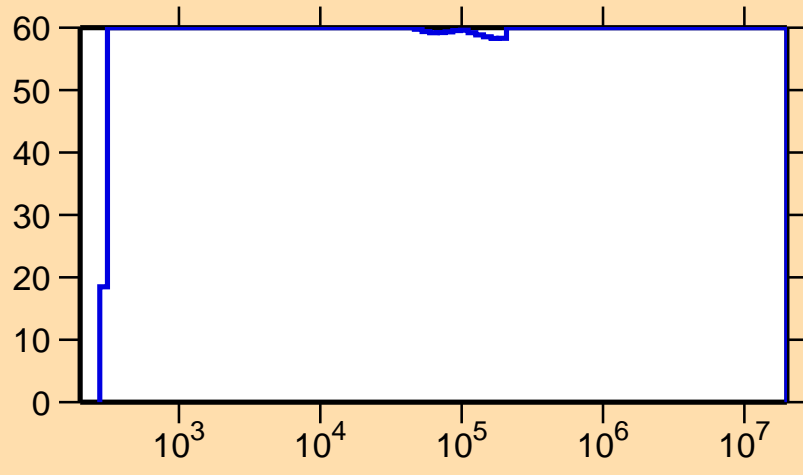
\Delta\sigma/\sigma vs. E for ^{144}\text{Pm}(n,p)
