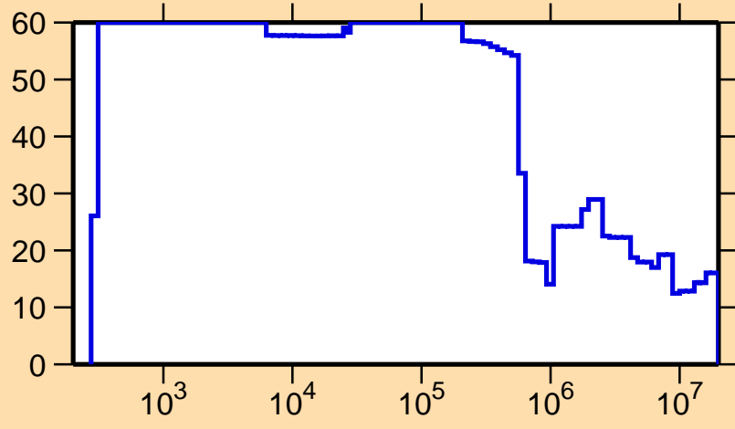
\Delta\sigma/\sigma vs. E for ^{144}\text{Pm}(n,el.)
