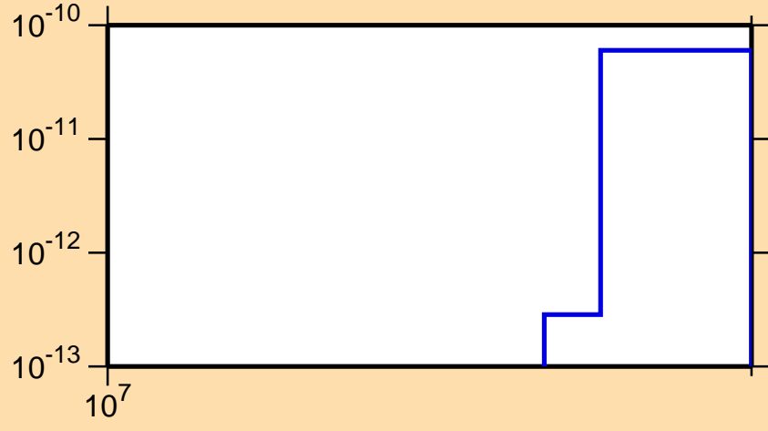
\sigma vs. E for ^{144}\text{Pm}(n,pt)
