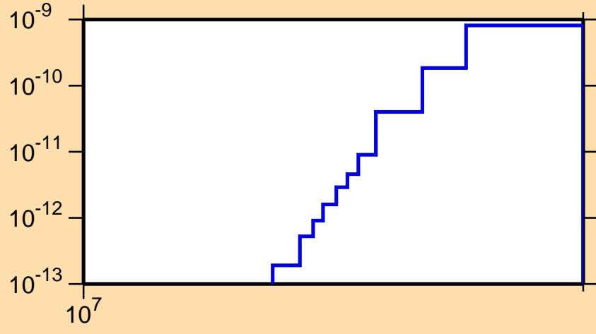
\sigma vs. E for ^{144}\text{Pm}(\text{mt117})
