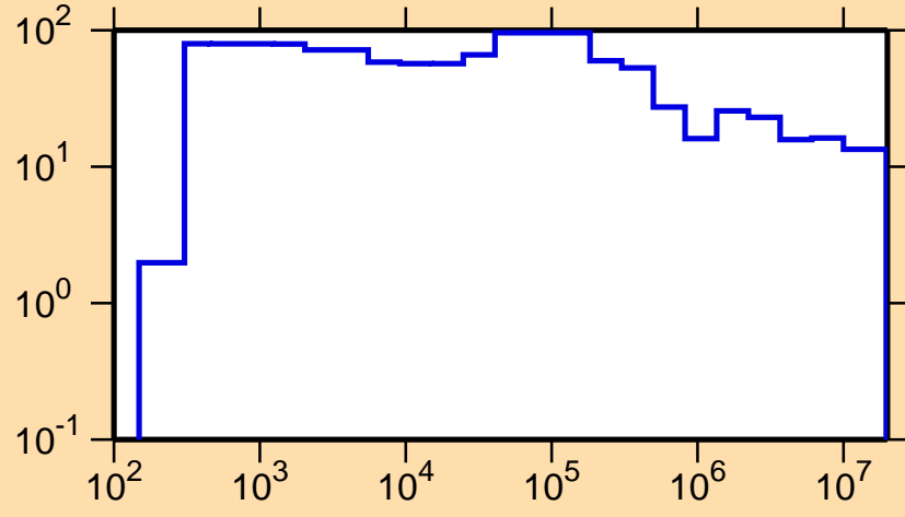
\Delta\sigma/\sigma vs. E for ^{144}\text{Pm}(n,el.)
