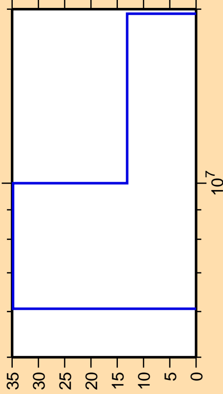
\Delta\sigma/\sigma vs. E for ^{144}\text{Pm}(n,2n)
