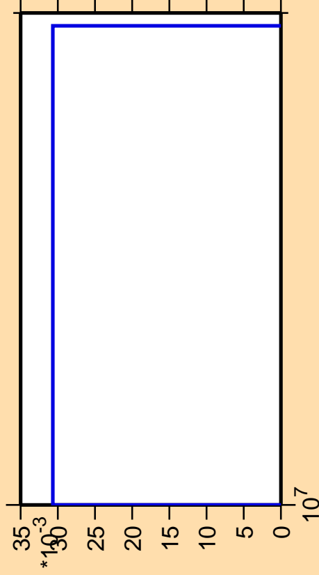
\Delta\sigma/\sigma vs. E for ^{144}\text{Pm}(n,pd)
