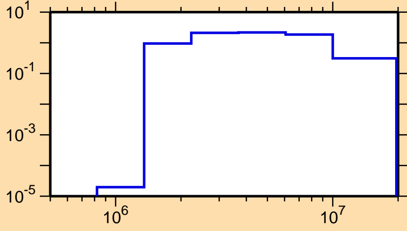
\sigma vs. E for ^{144}\text{Pm}(n,n\text{cont.})
