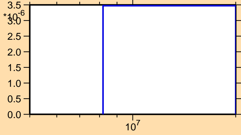
\sigma vs. E for ^{144}\text{Pm}(n,nd)
