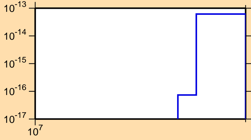
\sigma vs. E for ^{145}\text{Pm}(n,pd)
