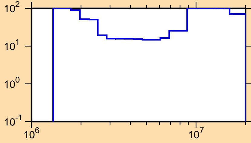
\Delta\sigma/\sigma vs. E for ^{145}\text{Pm}(n,n\text{cont.})
