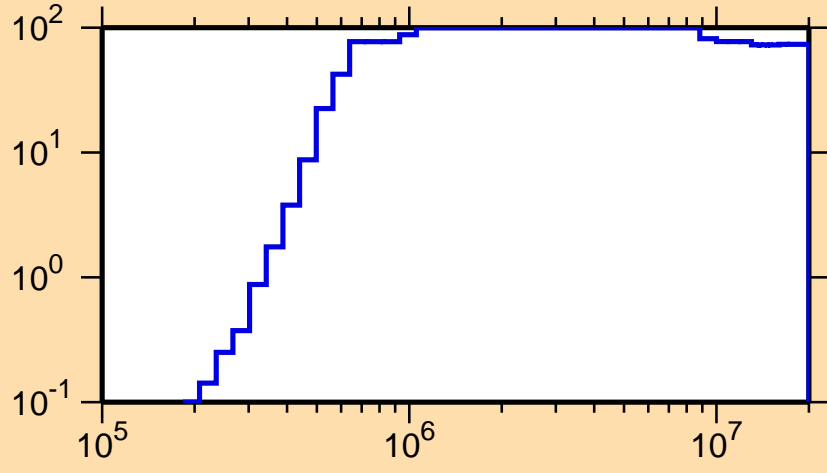
\Delta\sigma/\sigma vs. E for ^{145}\text{Pm}(n,p)
