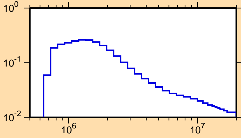
\sigma vs. E for ^{145}\text{Pm}(n,n_4)
