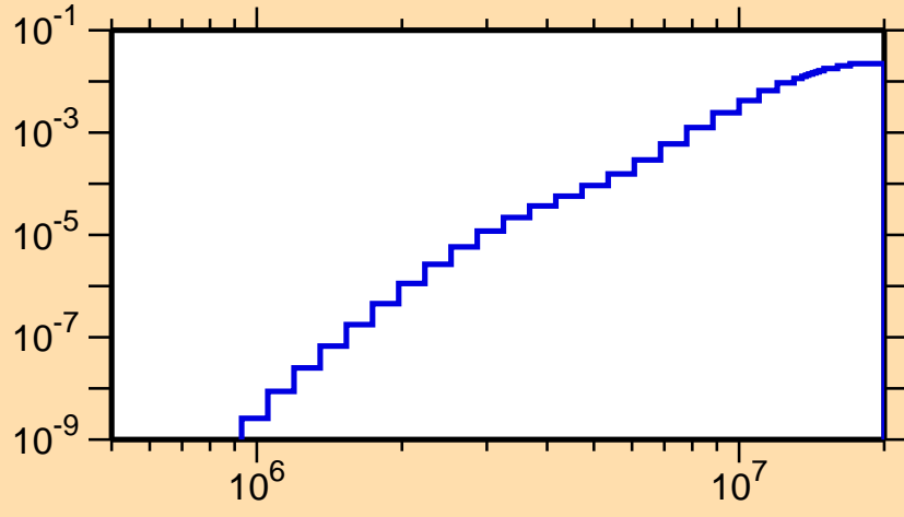
\sigma vs. E for ^{145}\text{Pm}(n,p)
