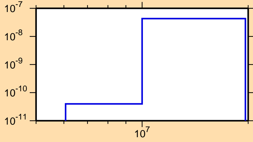
\sigma vs. E for ^{145}\text{Pm}(n,p\alpha)
