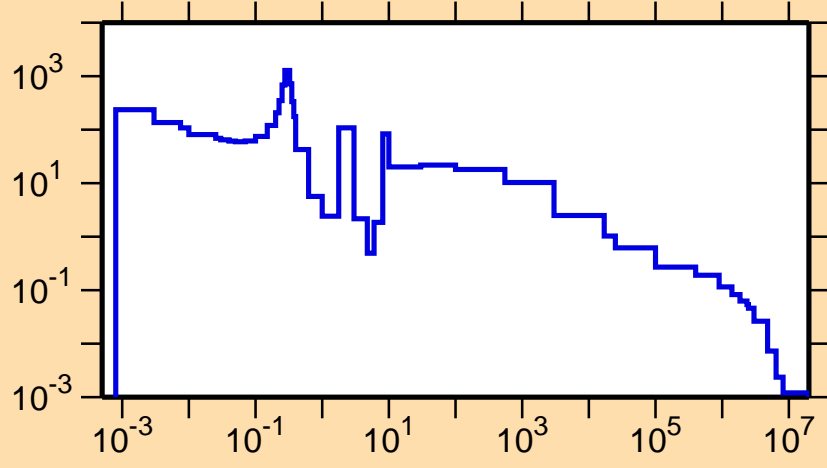
\sigma vs. E for ^{145}\text{Pm}(n,\gamma)
