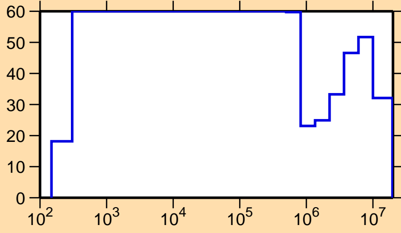
\Delta\sigma/\sigma vs. E for ^{146}\text{Pm}(n,el.)
