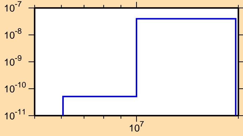
\sigma vs. E for ^{146}\text{Pm}(n,p\alpha)
