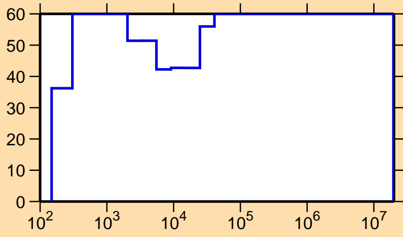
\Delta\sigma/\sigma vs. E for ^{146}\text{Pm}(n,\gamma)
