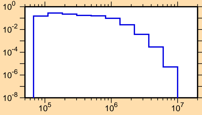
\sigma vs. E for ^{146}\text{Pm}(n,n_3)
