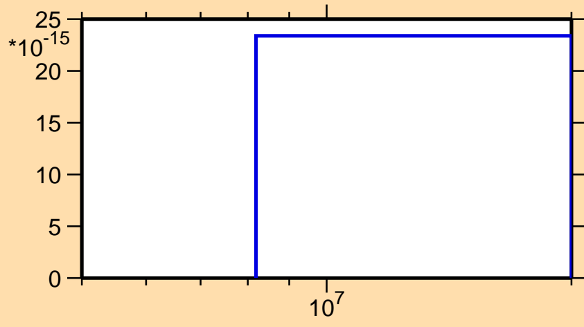
\sigma vs. E for ^{146}\text{Pm}(n,3n\alpha)
