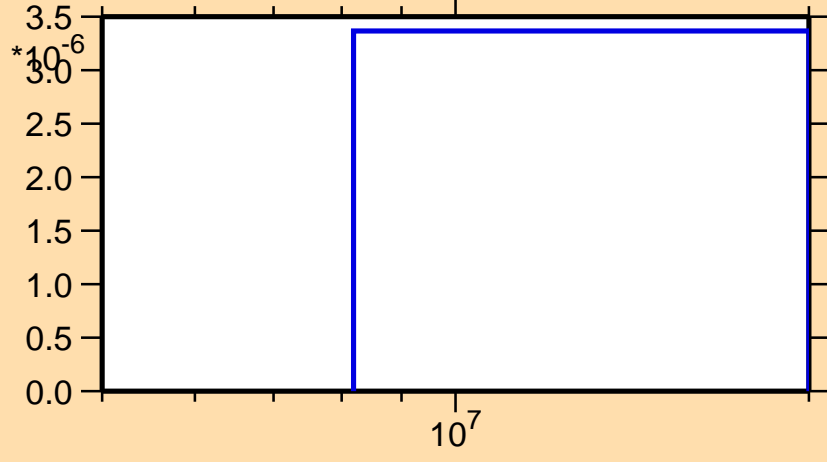
\sigma vs. E for ^{146}\text{Pm}(n,nd)
