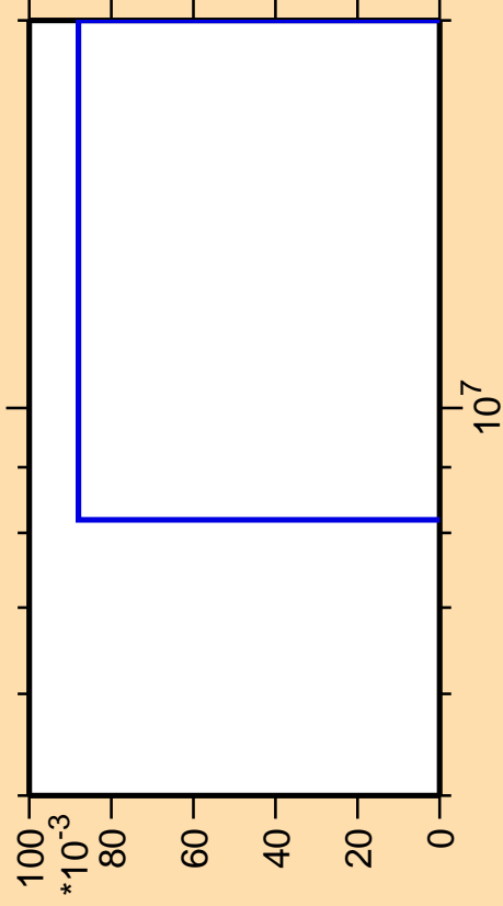
\Delta\sigma/\sigma vs. E for ^{146}\text{Pm}(n,3n\alpha)
