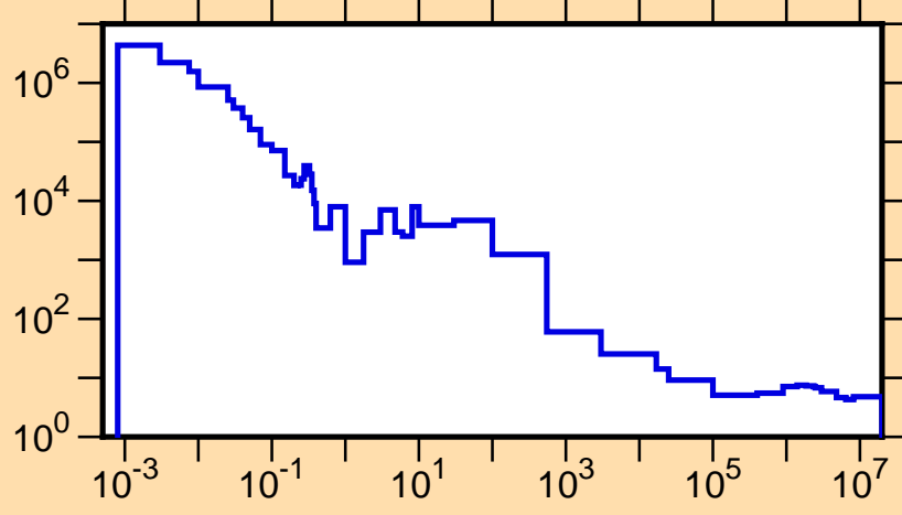
\sigma vs. E for ^{146}\text{Pm}(n,\text{tot.})
