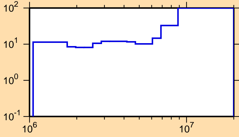
\Delta\sigma/\sigma vs. E for ^{147}\text{Pm}(n,n\text{cont.})
