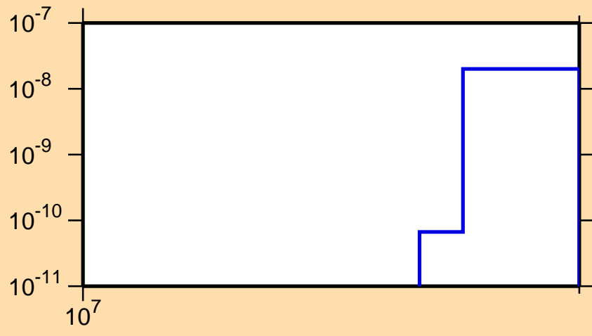
\sigma vs. E for ^{147}\text{Pm}(n,3n\alpha)
