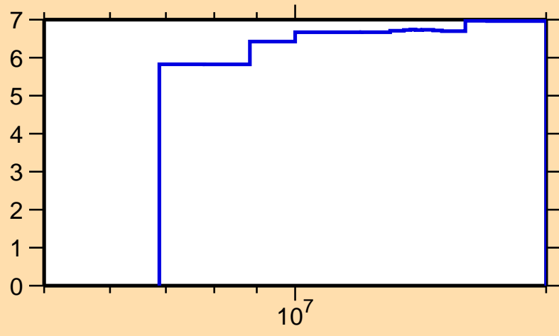
\Delta\sigma/\sigma vs. E for ^{147}\text{Pm}(n,\text{nonel.})
