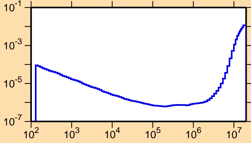
\sigma vs. E for ^{147}\text{Pm}(n,\alpha)
