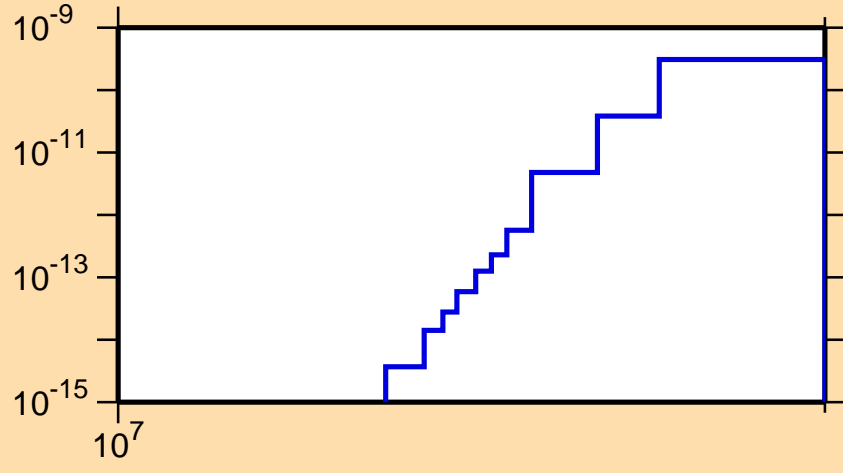
\sigma vs. E for ^{147}\text{Pm} (mt 45)
