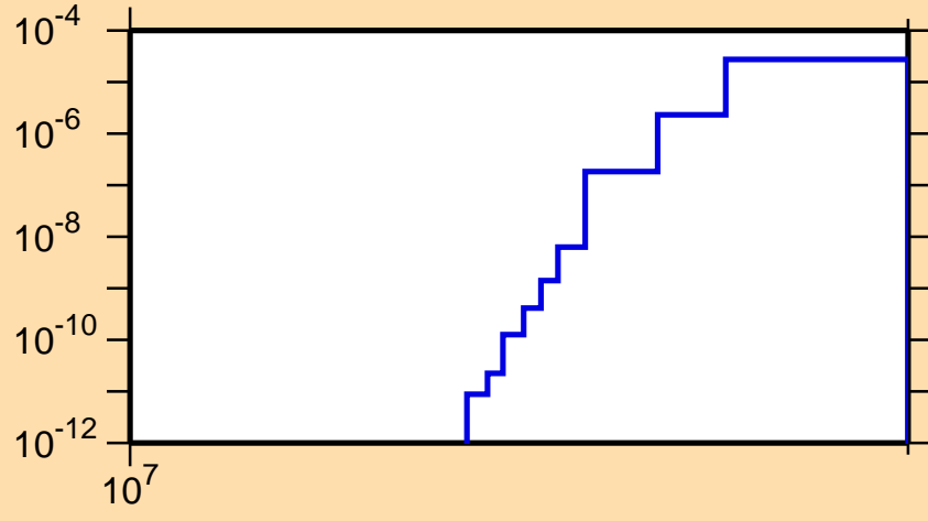
\sigma vs. E for ^{147}\text{Pm}(n,nd)
