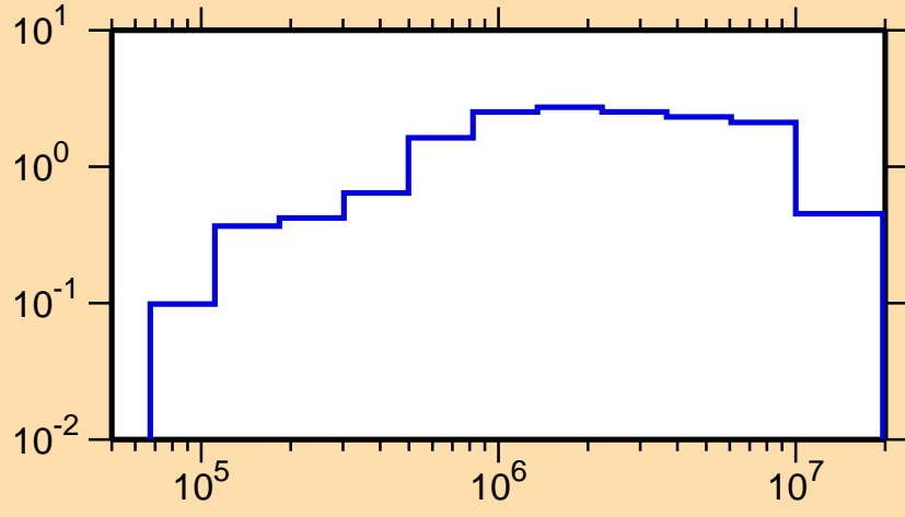
\sigma vs. E for ^{147}\text{Pm}(n,\text{inel.})
