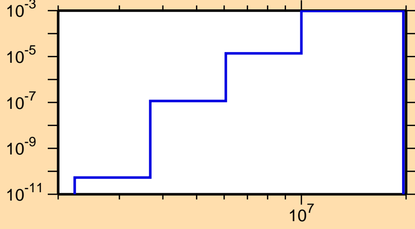
\sigma vs. E for ^{147}\text{Pm}(n,n\alpha)
