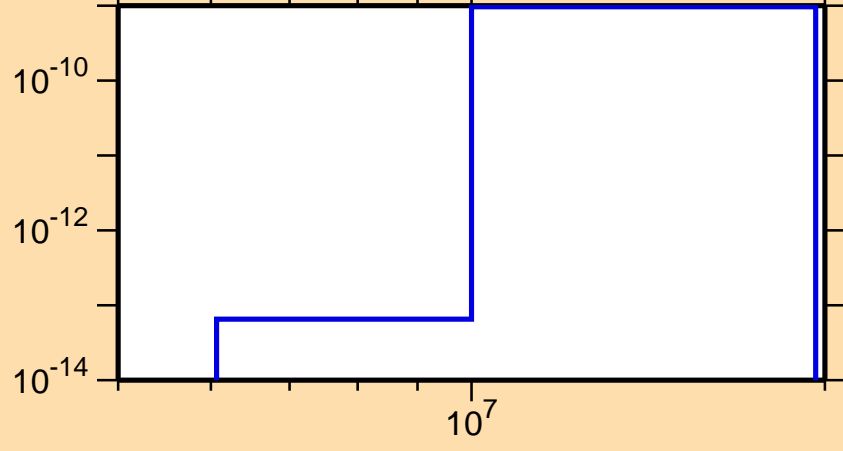
\sigma vs. E for ^{147}\text{Pm}(n,p\alpha)
