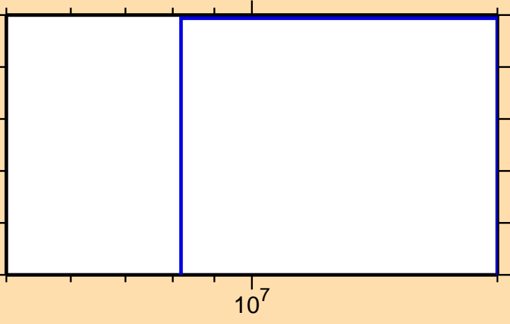
\sigma vs. E for ^{147}\text{Pm}(n,2np)
