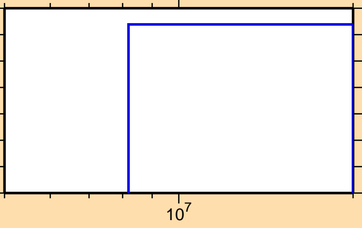
\sigma vs. E for ^{147}\text{Pm}(n,\text{He}3)
