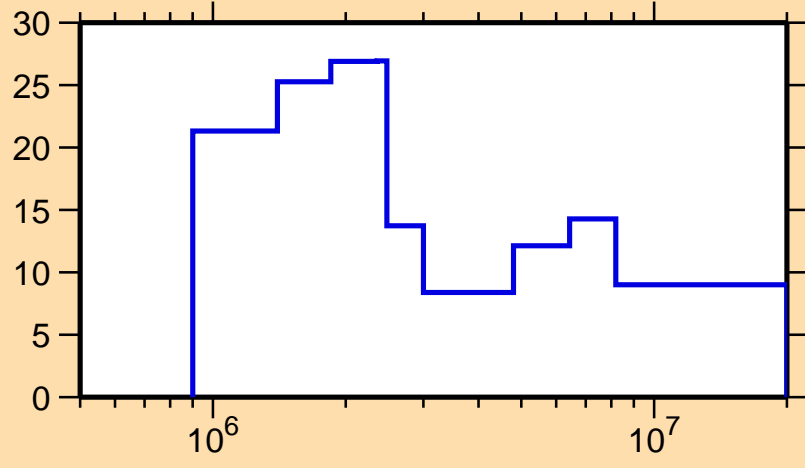
\Delta\sigma/\sigma vs. E for ^{147}\text{Pm}(n, tot.)
