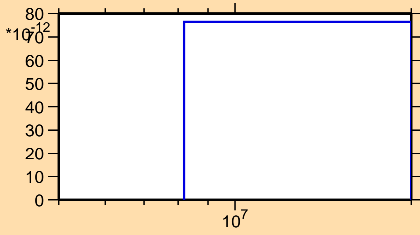
\sigma vs. E for ^{148}\text{Pm}(n,\text{He}3)
