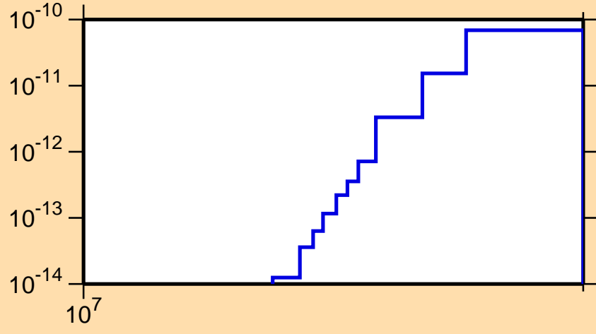
\sigma vs. E for ^{148}\text{Pm}(\text{mt117})
