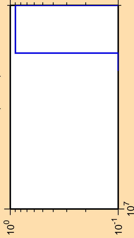
\Delta\sigma/\sigma vs. E for ^{148}\text{Pm} (mt 34)
