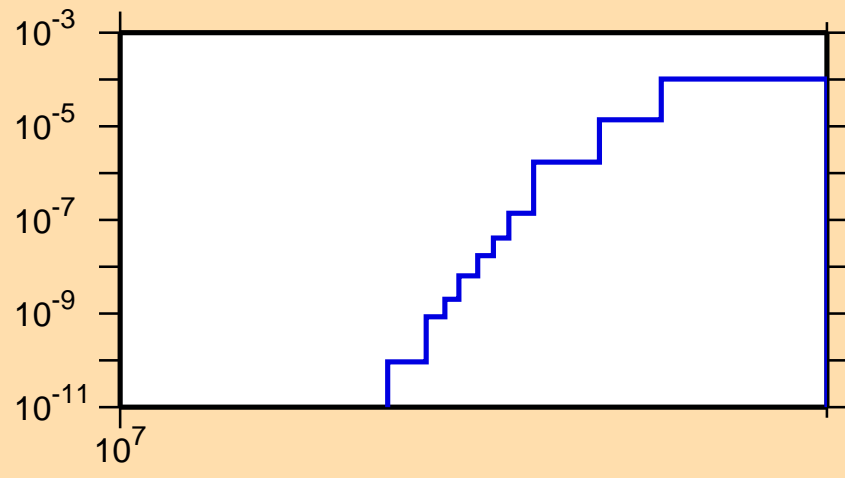
\sigma vs. E for ^{148}\text{Pm}(n,2np)
