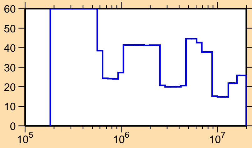
\Delta\sigma/\sigma vs. E for ^{148}\text{Pm}(n,el.)
