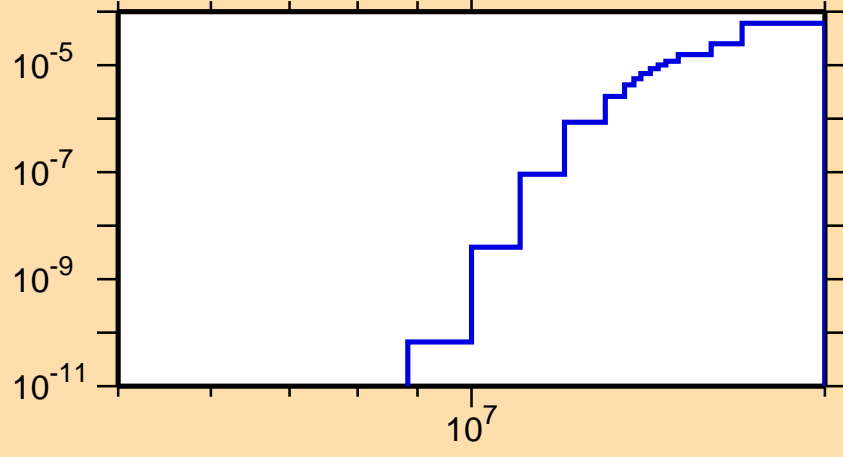
\sigma vs. E for ^{148}\text{Pm}(n,2n\alpha)
