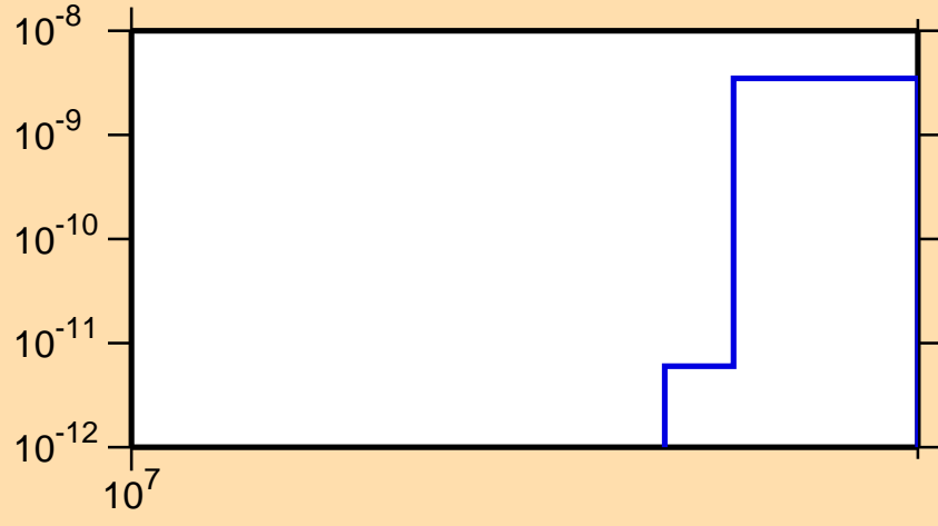
\sigma vs. E for ^{148}\text{Pm}(n,3n\alpha)
