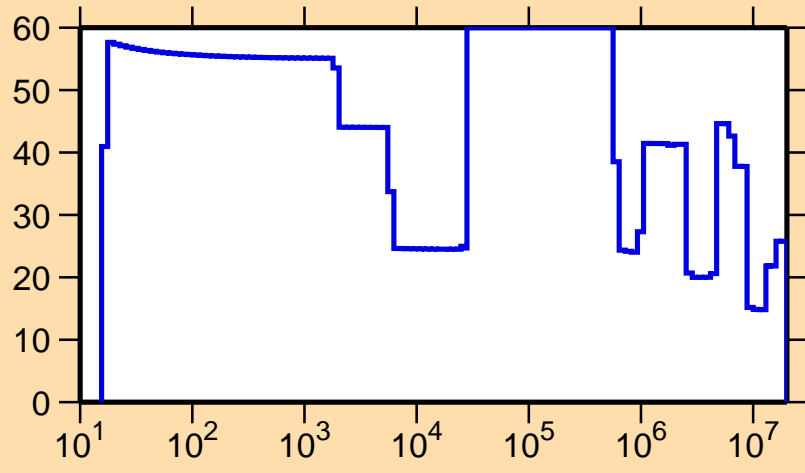
\Delta\sigma/\sigma vs. E for ^{148}\text{Pm}(n,\text{el.})
