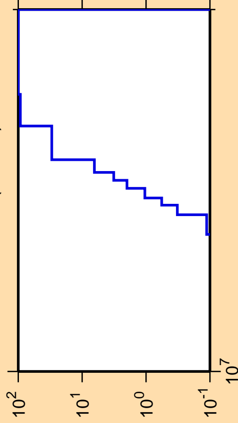
\Delta\sigma/\sigma vs. E for ^{148}\text{Pm}(\text{mt117})
