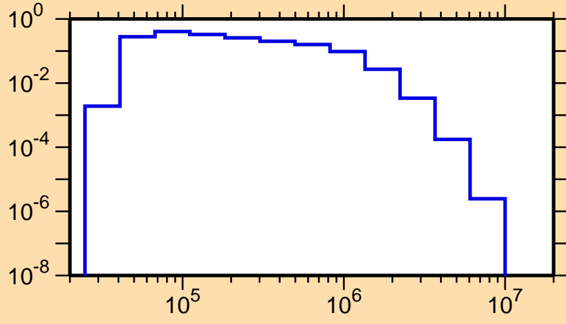
\sigma vs. E for ^{148}\text{Pm}(n,n_4)
