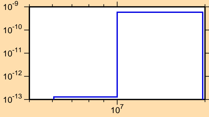
\sigma vs. E for ^{148}\text{Pm}(n,p\alpha)
