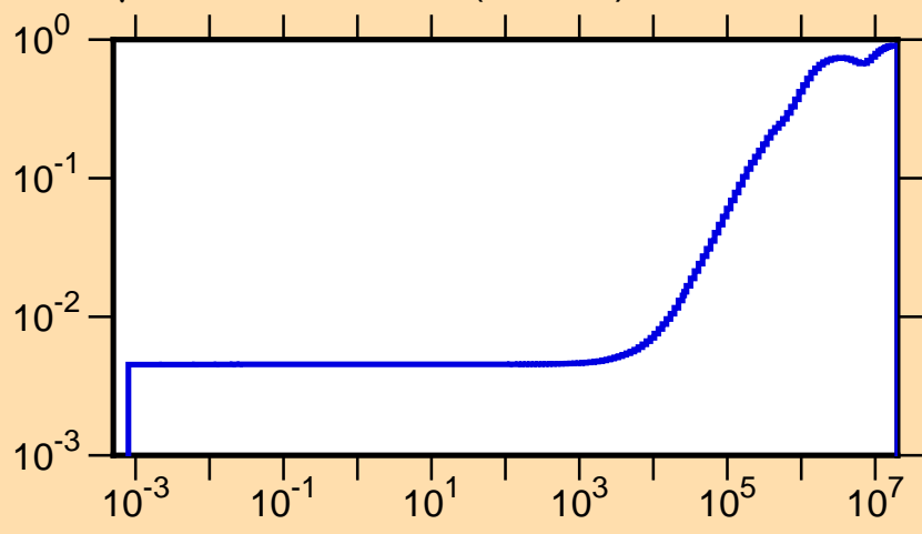
\mu vs. E for ^{149}\text{Pm}(\text{mt251})
