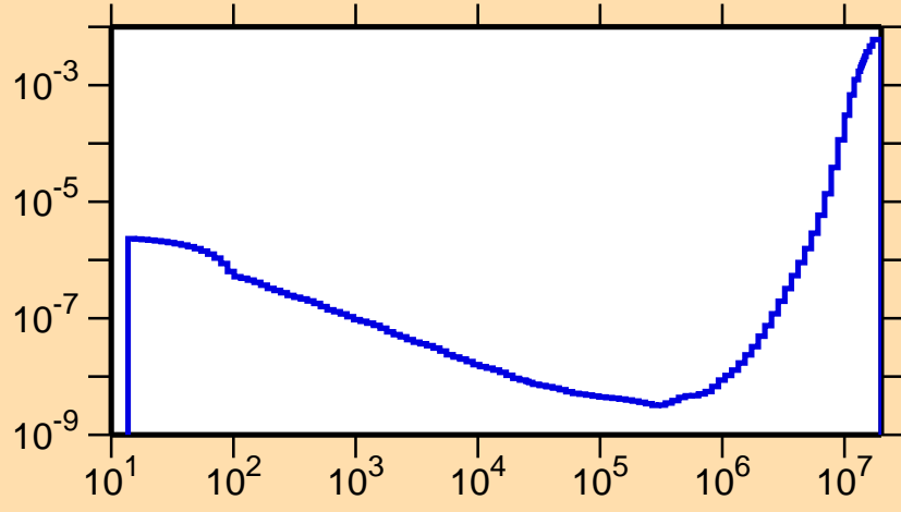
\sigma vs. E for ^{149}\text{Pm}(n,\alpha)
