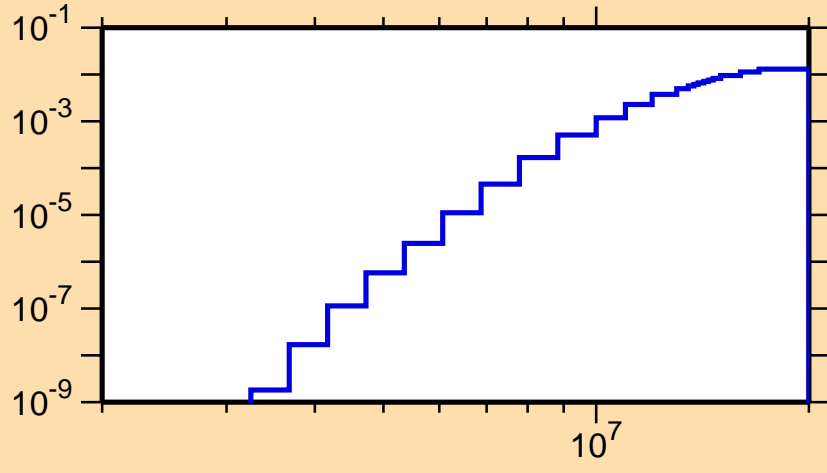
\sigma vs. E for ^{149}\text{Pm}(n,p)
