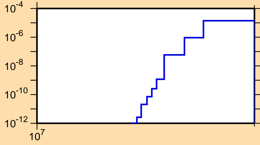
\sigma vs. E for ^{149}\text{Pm}(n,nd)
