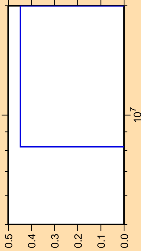
\Delta\sigma/\sigma vs. E for ^{149}\text{Pm} (mt 45)
