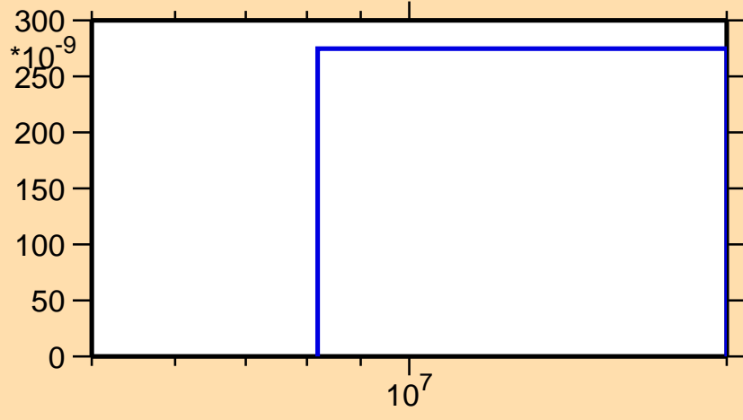
\sigma vs. E for ^{149}\text{Pm}(n,2n\alpha)
