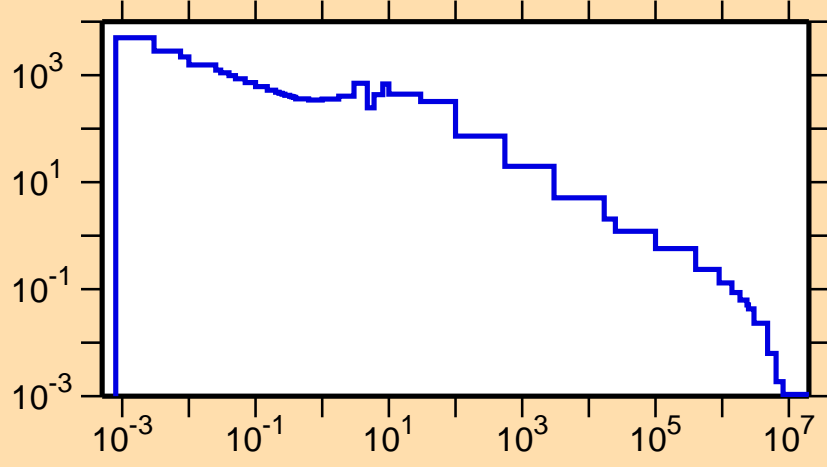
\sigma vs. E for ^{149}\text{Pm}(n,\gamma)
