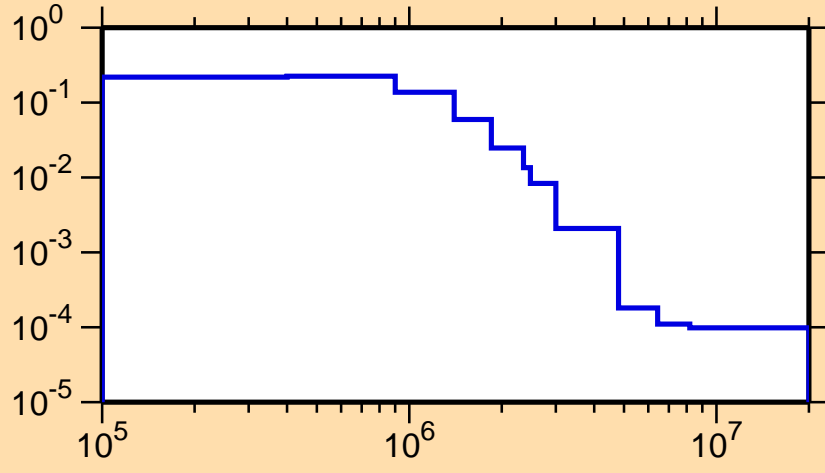
\sigma vs. E for ^{149}\text{Pm}(n,n_1)
