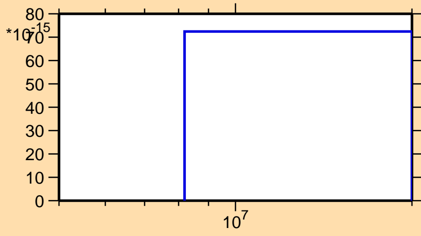
\sigma vs. E for ^{149}\text{Pm} (mt 45)
