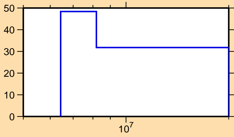
\Delta\sigma/\sigma vs. E for ^{149}\text{Pm}(n,el.)
