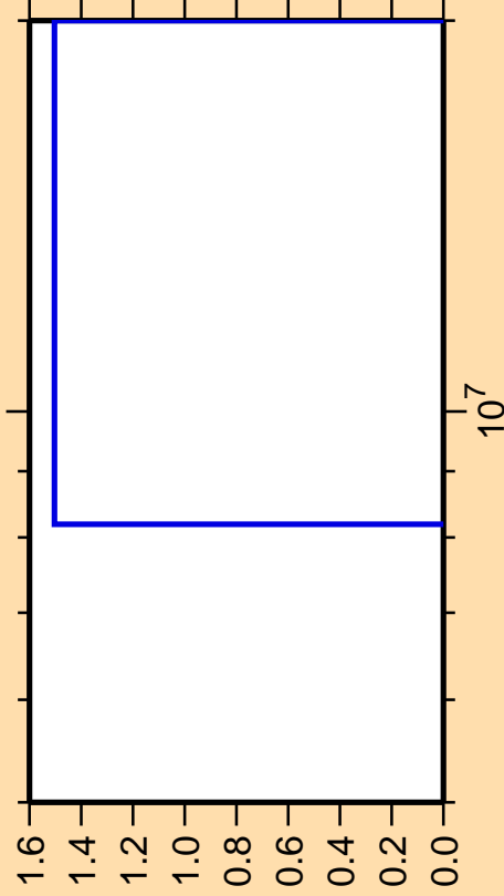
\Delta\sigma/\sigma vs. E for ^{149}\text{Pm}(\text{mt117})
