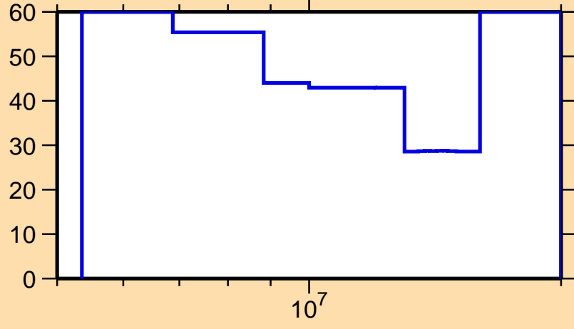
\Delta\sigma/\sigma vs. E for ^{150}\text{Pm}(n,2n)
