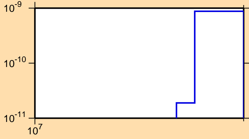
\sigma vs. E for ^{150}\text{Pm}(n,\text{He}3)
