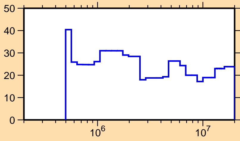
\Delta\sigma/\sigma vs. E for ^{150}\text{Pm}(n,\text{tot.})
