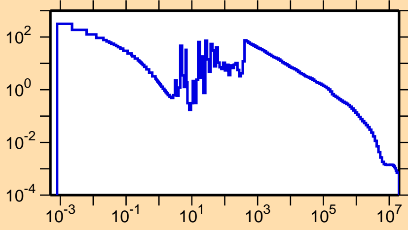
\sigma vs. E for ^{150}\text{Pm}(n,\gamma)
