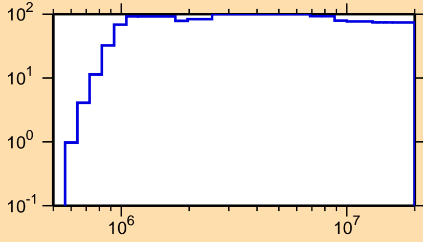
\Delta\sigma/\sigma vs. E for ^{150}\text{Pm}(n,p)
