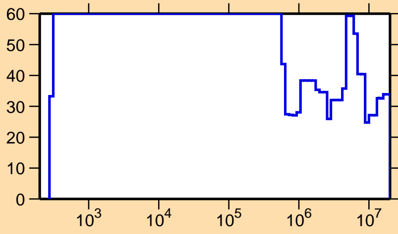
\Delta\sigma/\sigma vs. E for ^{150}\text{Pm}(n,\text{el.})
