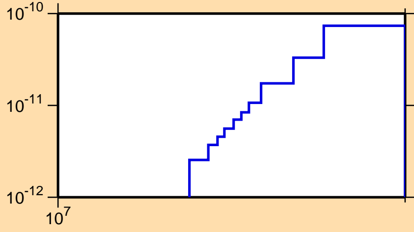
\sigma vs. E for ^{150}\text{Pm}(n,p\alpha)
