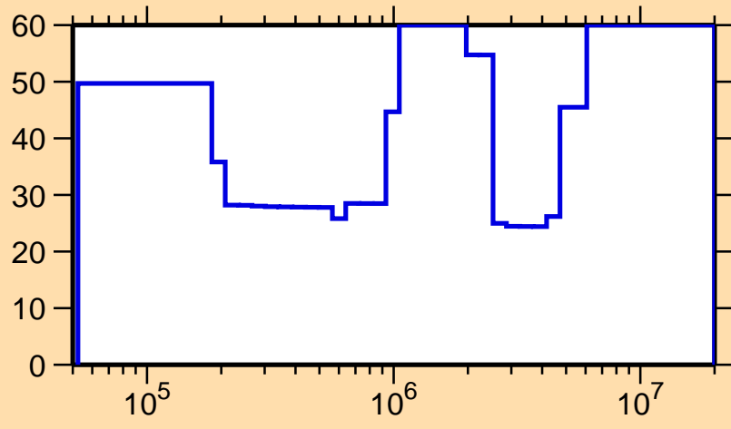
\Delta\sigma/\sigma vs. E for ^{150}\text{Pm}(n,\text{inel.})
