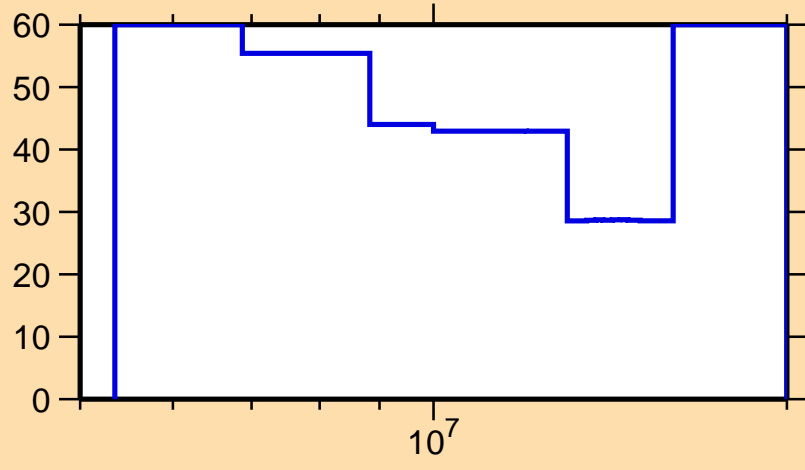
\Delta\sigma/\sigma vs. E for ^{150}\text{Pm}(n,2n)
