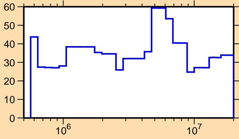
\Delta\sigma/\sigma vs. E for ^{150}\text{Pm}(n,e.l.)
