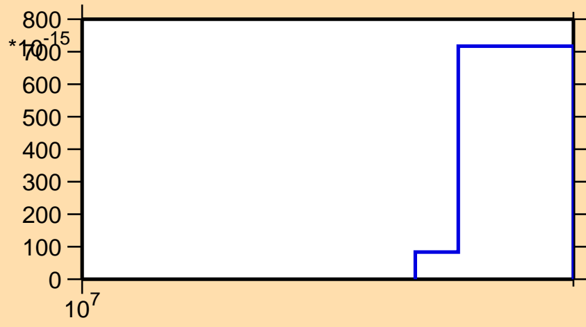
\sigma vs. E for ^{150}\text{Pm}(\text{mt117})
