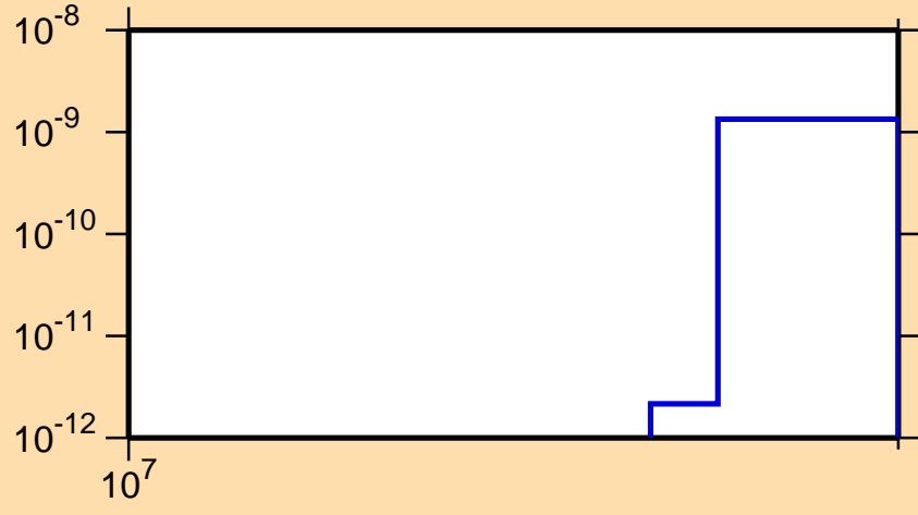
\sigma vs. E for ^{150}\text{Pm}(n,3n\alpha)
