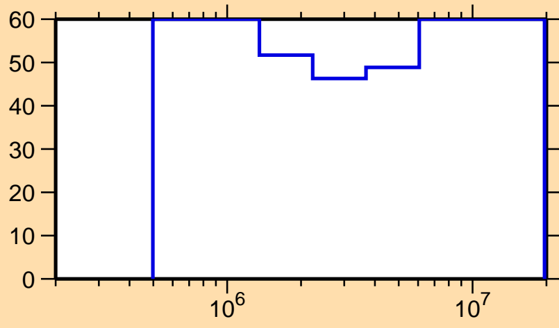
\Delta\sigma/\sigma vs. E for ^{150}\text{Pm}(n,n\text{cont.})
