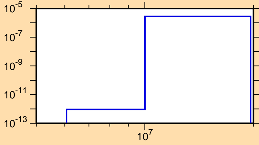
\sigma vs. E for ^{150}\text{Pm}(n,2n\alpha)
