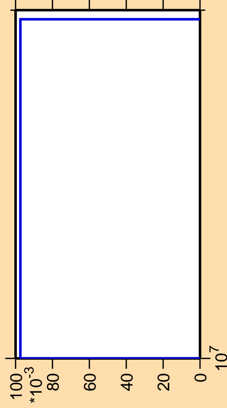
\Delta\sigma/\sigma vs. E for ^{150}\text{Pm}(\text{mt117})
