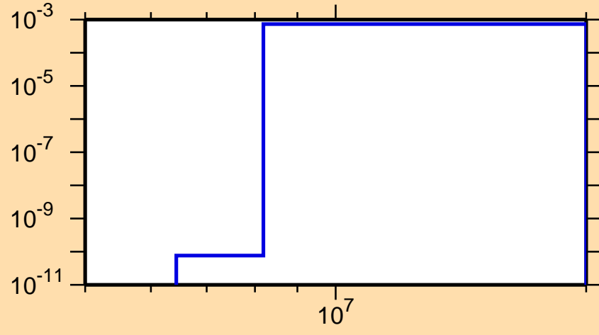
\sigma vs. E for ^{150}\text{Pm}(n,d)
