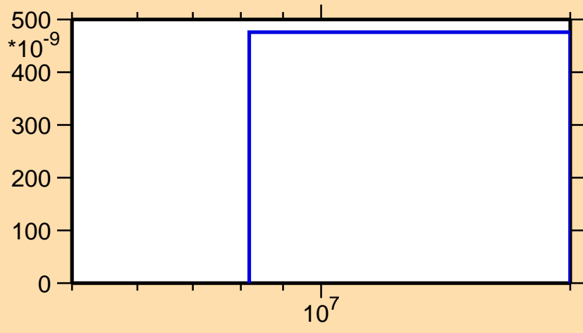
\sigma vs. E for ^{150}\text{Pm}(n,nt)
