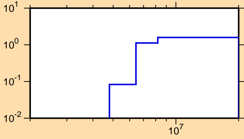
\sigma vs. E for ^{150}\text{Pm}(n,2n)
