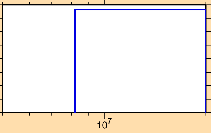
\sigma vs. E for ^{150}\text{Pm} (mt 11)
