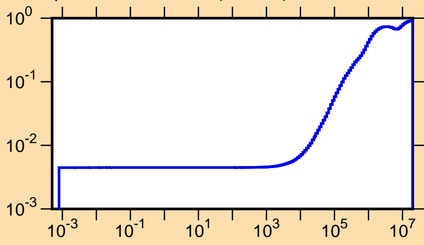
\mu vs. E for ^{151}\text{Pm}(\text{mt251})
