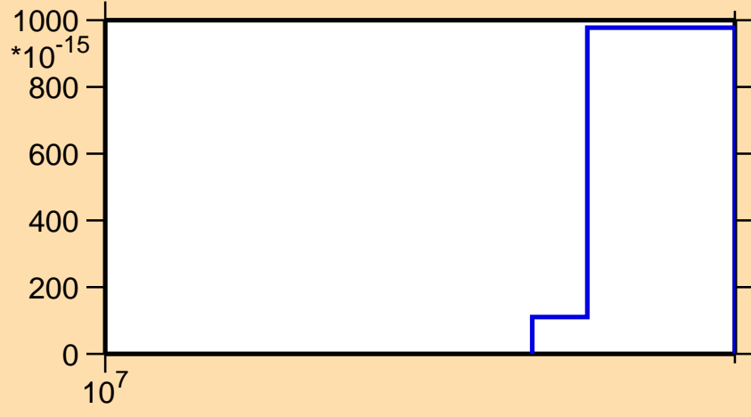
\sigma vs. E for ^{151}\text{Pm}(n,p\alpha)
