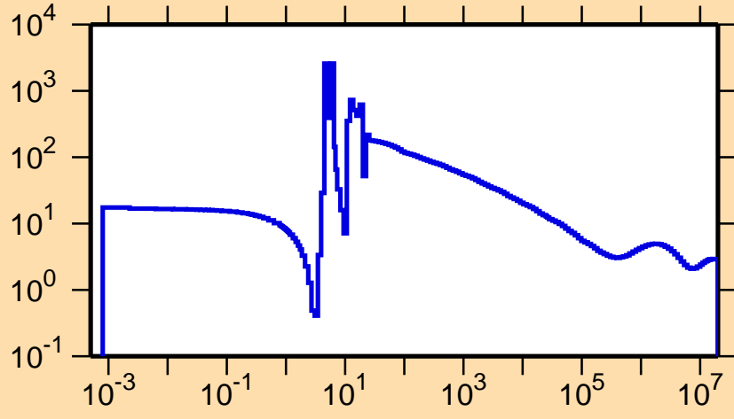
\sigma vs. E for ^{151}\text{Pm}(n,\text{el.})
