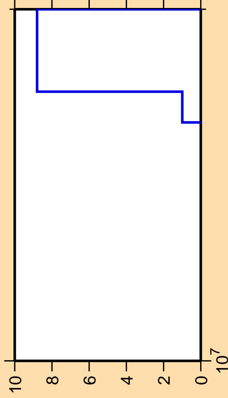
\Delta\sigma/\sigma vs. E for ^{151}\text{Pm}(n,p\alpha)
