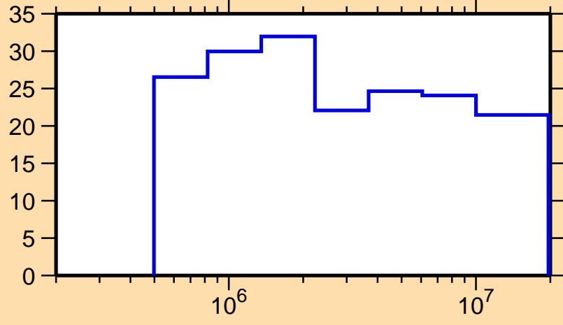
\Delta\sigma/\sigma vs. E for ^{151}\text{Pm}(n,tot.)
