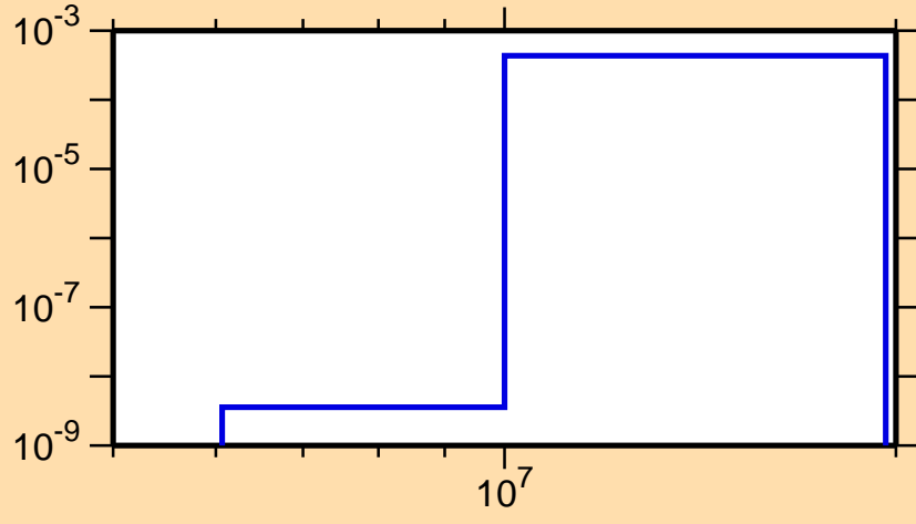
\sigma vs. E for ^{151}\text{Pm}(n,d)
