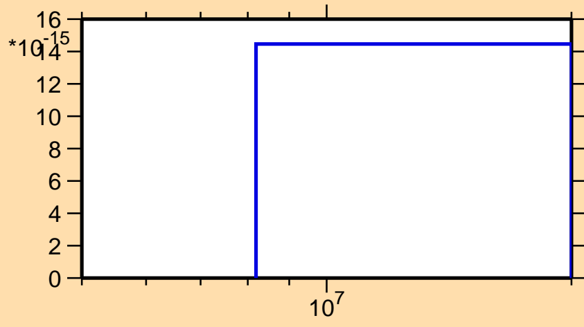
\sigma vs. E for ^{151}\text{Pm}(n,p\alpha)
