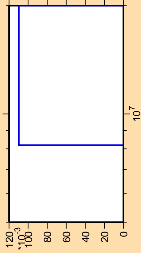
\Delta\sigma/\sigma vs. E for ^{151}\text{Pm}(n,p\alpha)
