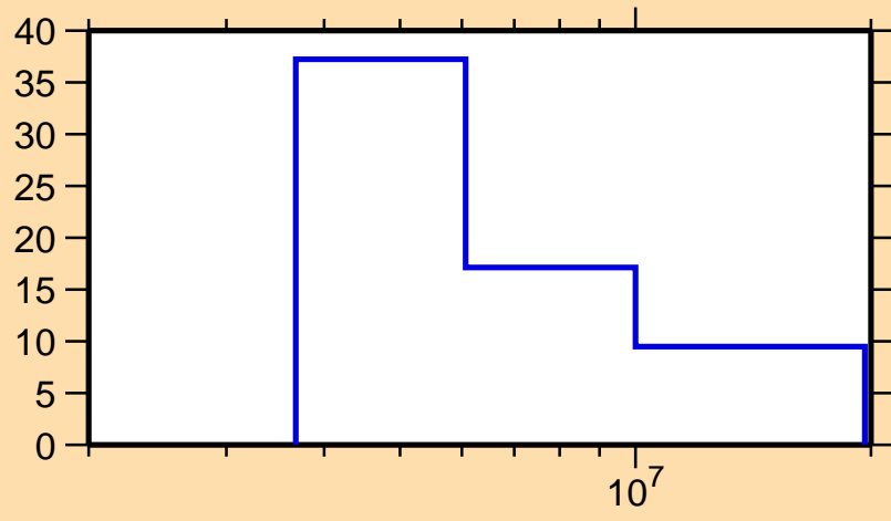
\Delta\sigma/\sigma vs. E for ^{152}\text{Pm}(n,el.)
