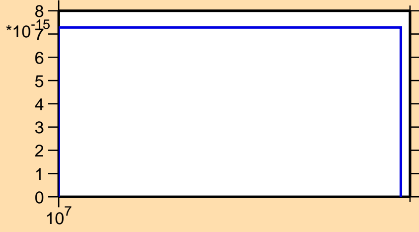
\sigma vs. E for ^{152}\text{Pm}(n,3n\alpha)
