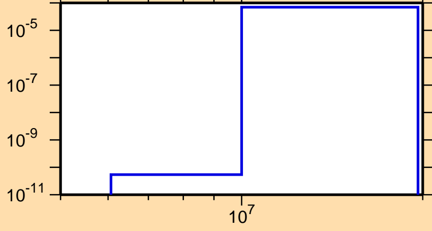
\sigma vs. E for ^{152}\text{Pm}(n,t)
