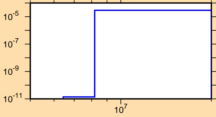
\sigma vs. E for ^{152}\text{Pm}(n,\alpha)
