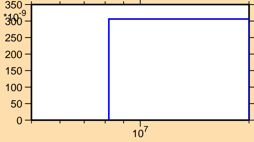
\sigma vs. E for ^{152}\text{Pm}(n,nd)
