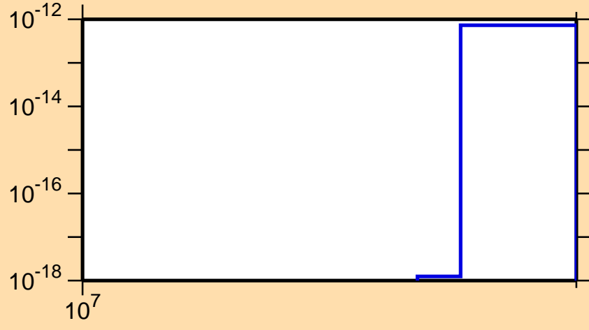
\sigma vs. E for ^{152}\text{Pm}(n,3n\alpha)
