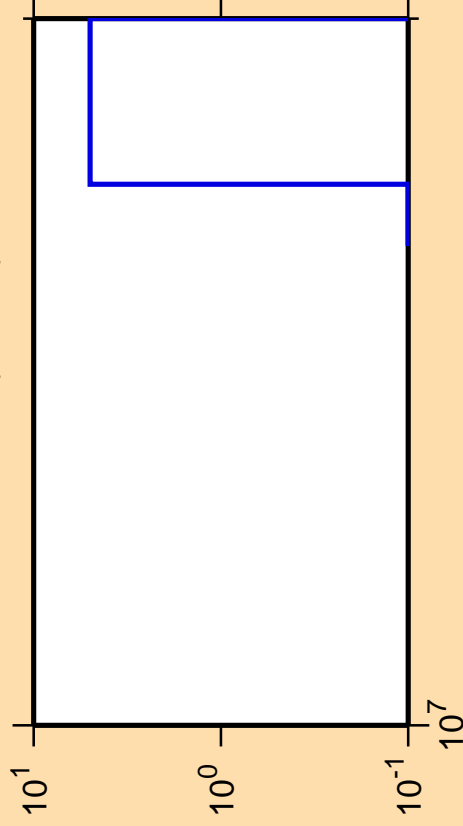
\Delta\sigma/\sigma vs. E for ^{152}\text{Pm}(n,3n\alpha)
