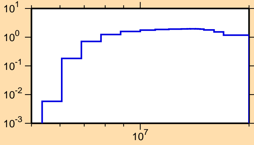
\sigma vs. E for ^{152}\text{Pm}(n,2n)
