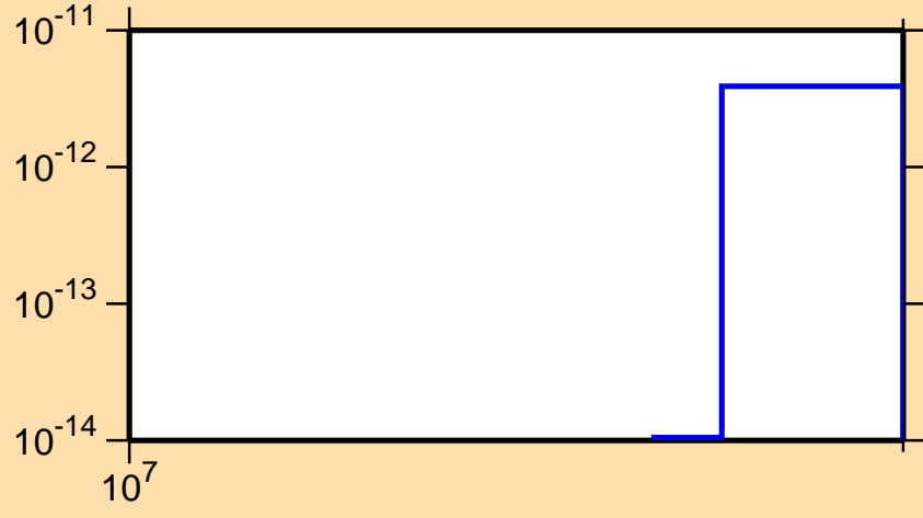
\sigma vs. E for ^{152}\text{Pm}(n,\text{He}3)
