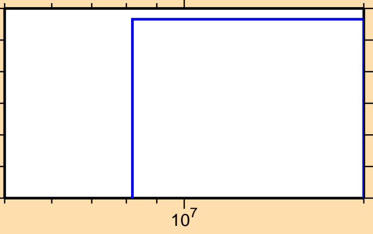
\sigma vs. E for ^{152}\text{Pm}(n,np)
