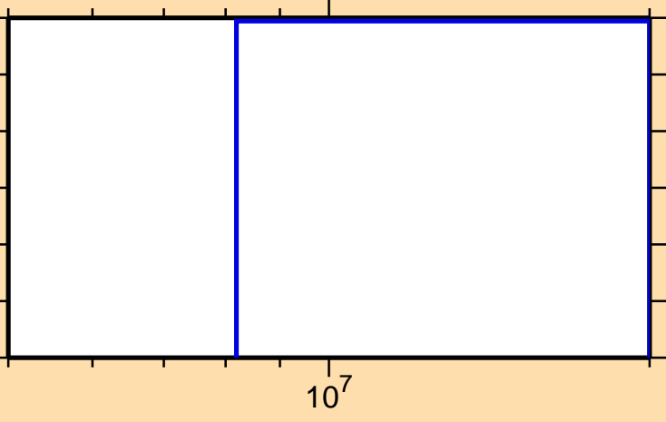
\sigma vs. E for ^{152}\text{Pm}(n,3n\alpha)
